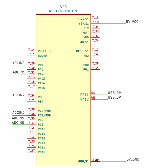
NUCLEO-F401RE DEVELOPMENT BOARD. POWER THE BOARD USING USB
