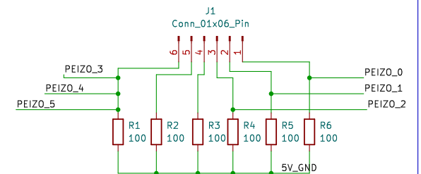
EXTERNAL_CONNECTORS FOR PEIZO
