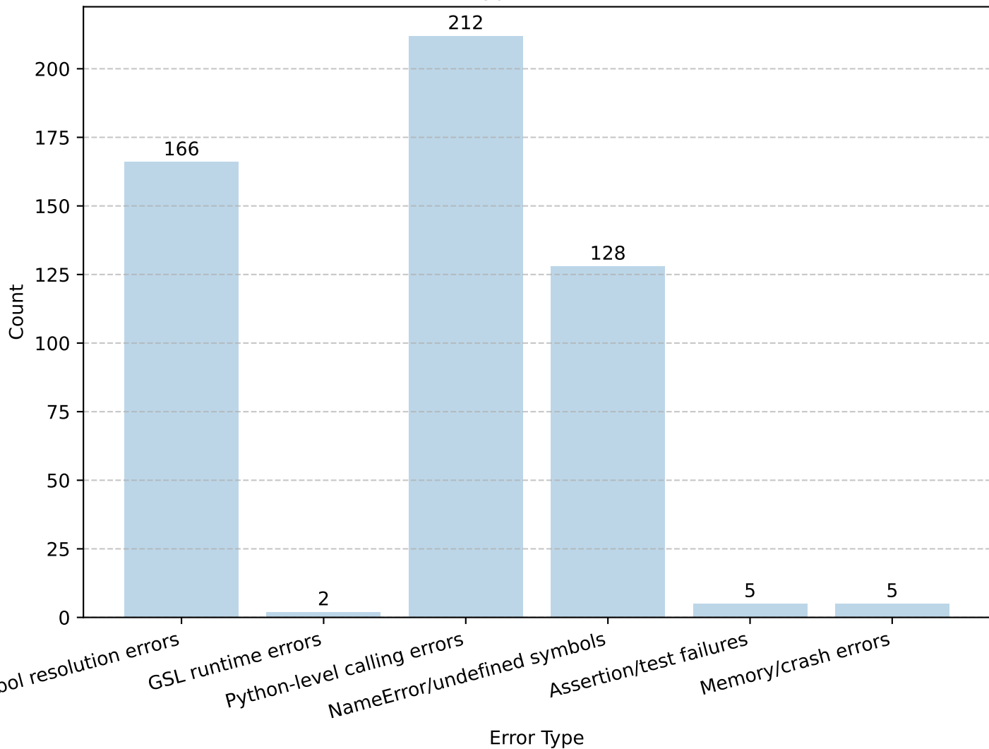
Error Type Distribution
