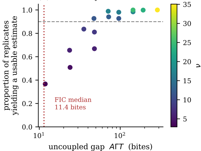
(A) estimability
