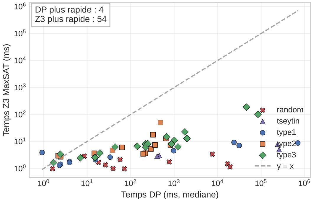
Temps de resolution DP vs Z3 (MaxSAT, log-log)
