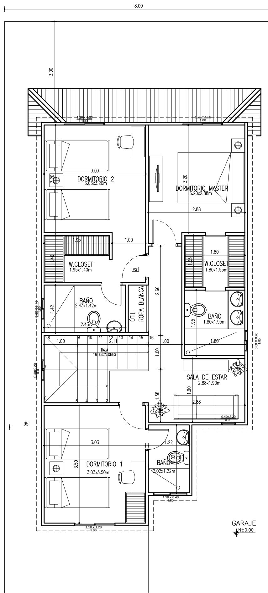
PLANTA ALTA AREA: 67.65m 2
