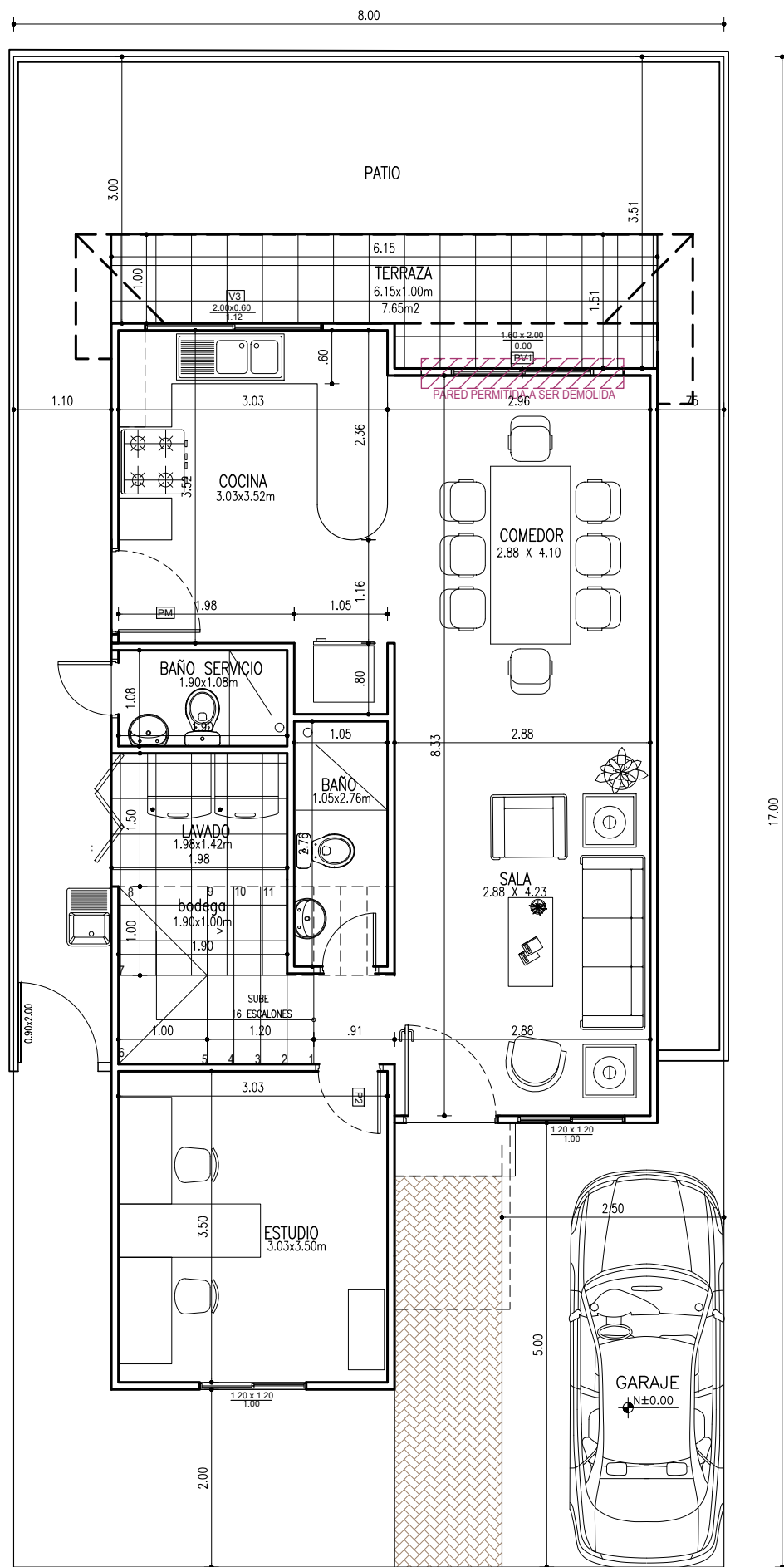
PLANTA BAJA AREA: 71.07m 2
