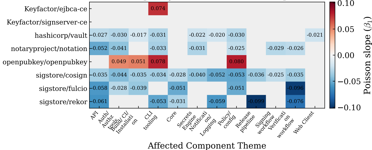
Poisson Time Slopes by Tool and Affected Component Theme
