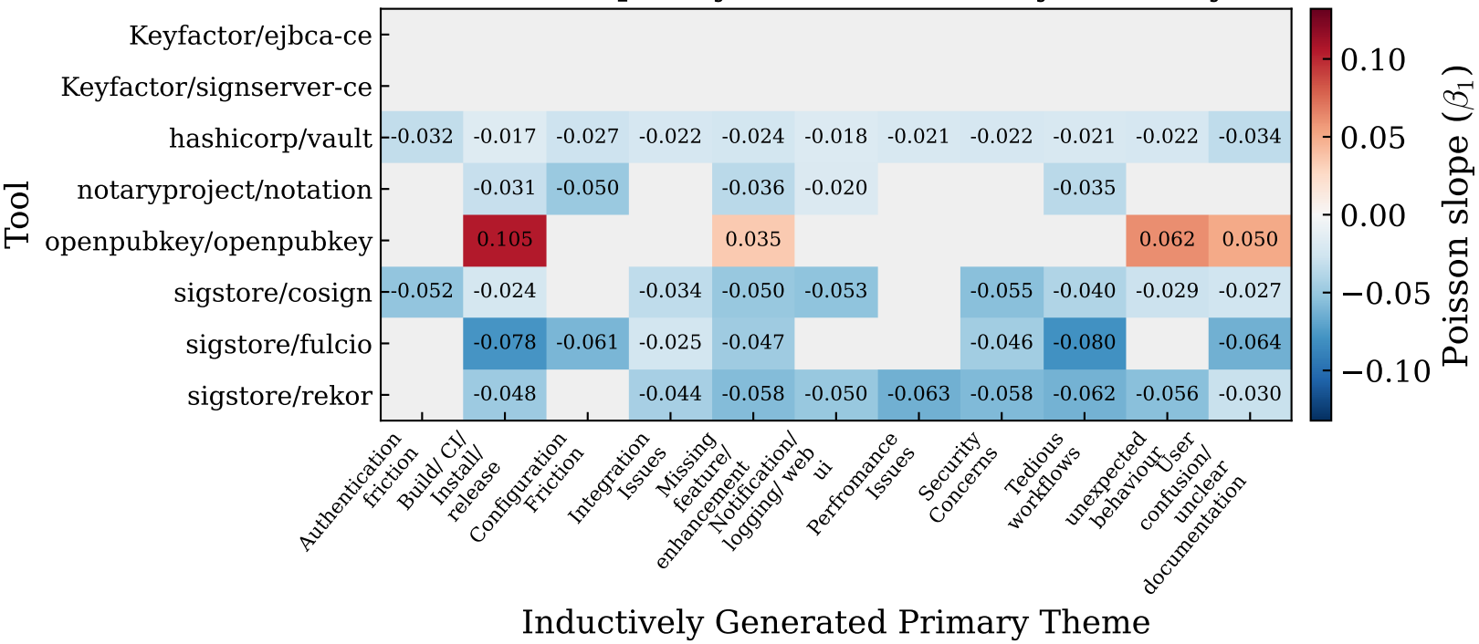
Poisson Time Slopes by Tool and Primary Usability Theme
