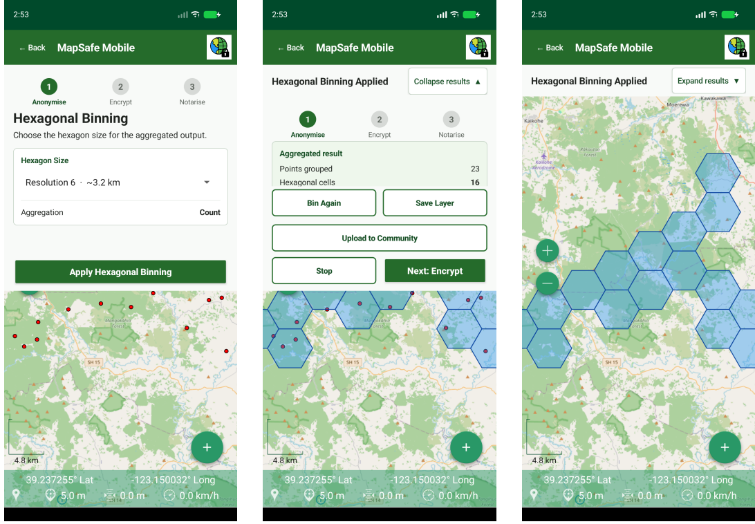
(a) Resolution 6 selected for the original points; the displayed 3.2 km text is the legacy H3 3.x estimate.
