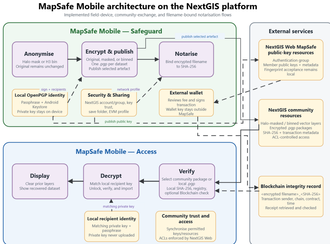
Figure 1.: MapSafe Mobile architecture. Sensitive processing occurs on the field device; NextGIS Web supports community membership, public-key exchange, and protected-resource distribution; an optional EVM record independently binds the encrypted package filename to its digest.
