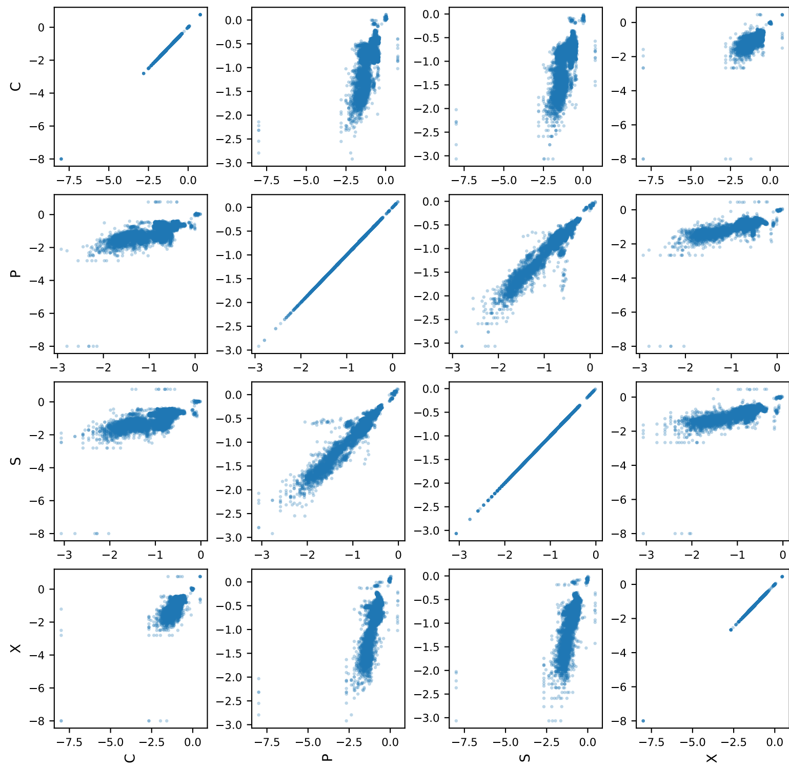
patristic distance scatter matrix. Log-10 transformed
