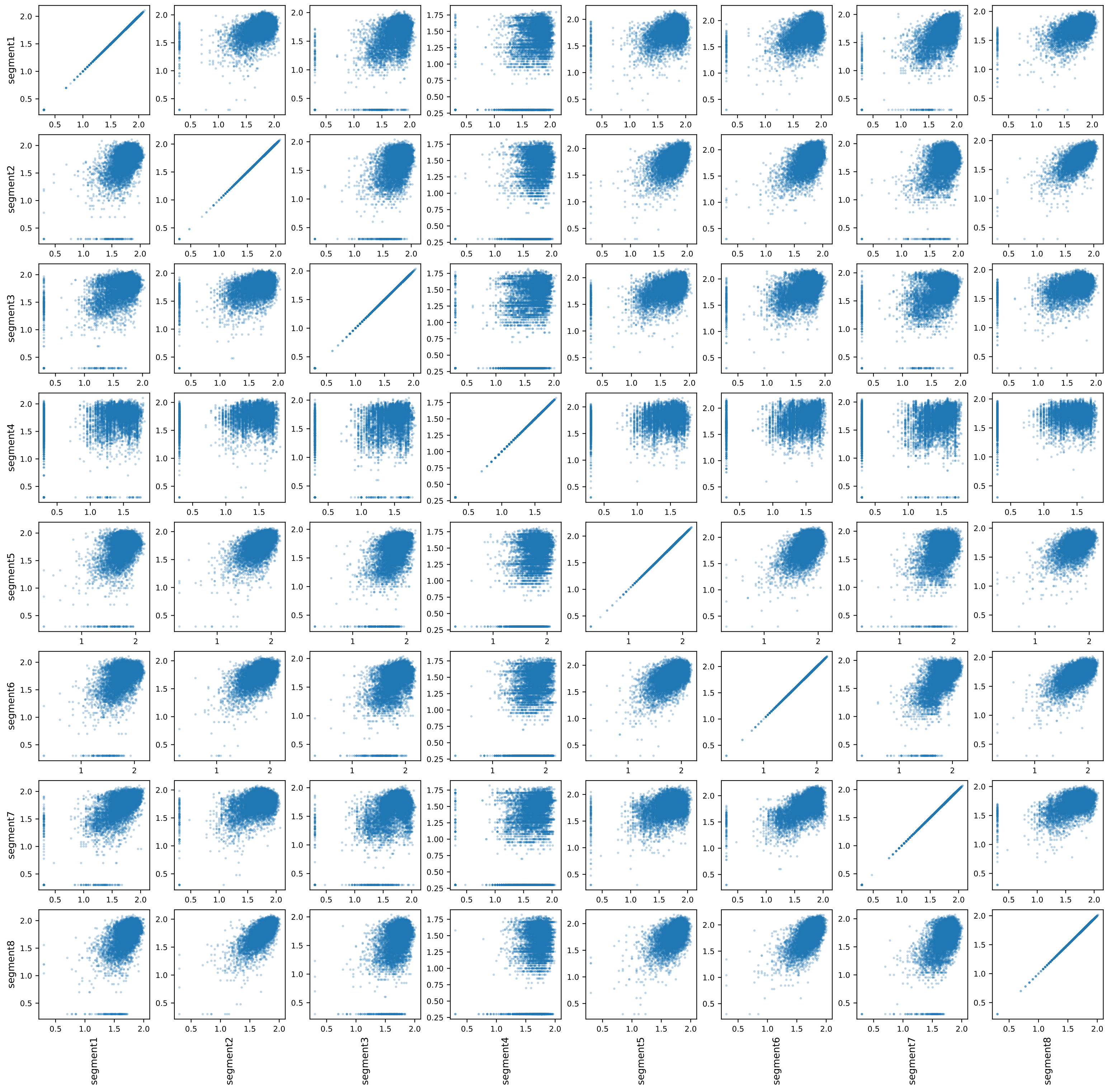
topo distance scatter matrix. Log-10 transformed
