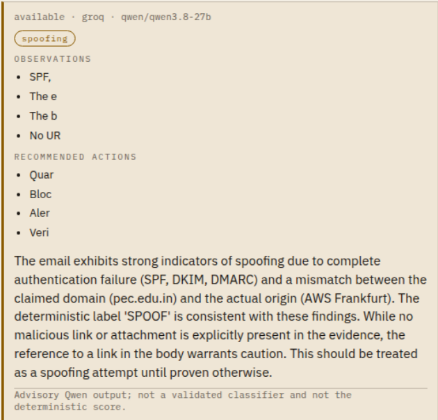
Figure 7 — Qwen notes (same Groq model). Wording class already went into the stamp as bounded NLP points.
