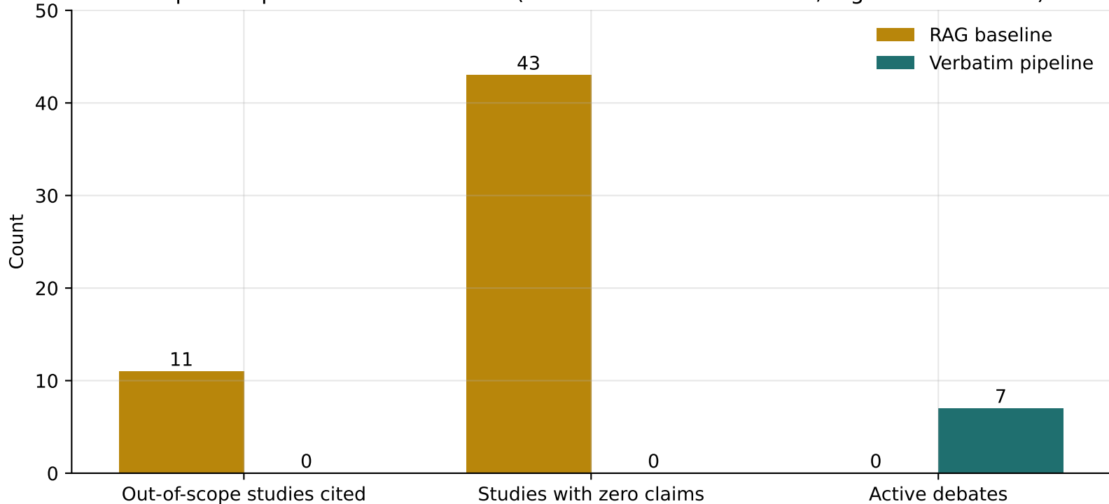
Corpus-scope & debate structure (lower is better for left two, higher for debates)
