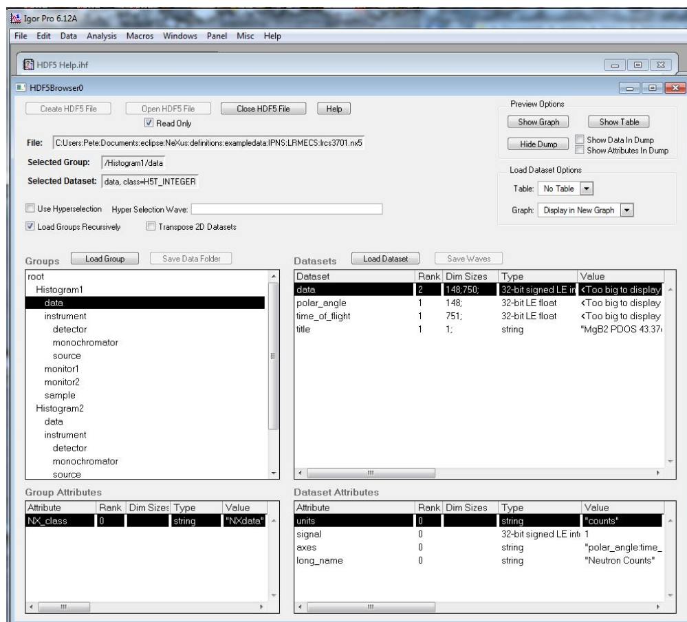
Fig. 12: LRMECS lrcs3701 data: IgorPro HDFBrowser dialog
