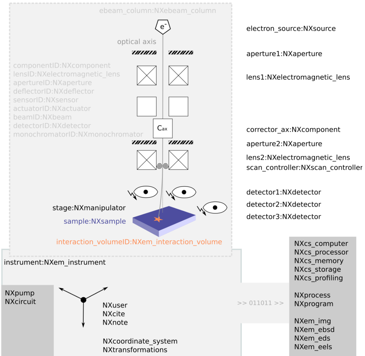
Fig. 1 - an example for an SEM The instrument is constructed from a so-called column, a housing for all technical components such as the electron source, the lenses, like here shown a condenser and an objective lens, respective apertures, and further components, like a stigmator to correct for axial image distortions. The trajectory of the electron beam along the optical axis is simplified for illustrative purposes. In summary, the sample is illuminated by an electron beam that is guided along the optical axis through and past a set of components. A scan controller is used to deflect this beam to illuminate specific locations on the sample surface. In response to the electron-beam sample interaction an interaction volume is formed. Different types of signals are generated that are picked up by different types of detectors. Three detectors are shown as an example. Apart from the column, an SEM has further components: The base classes that are used for modeling these are listed in the lower part of the figure. These document pumps and other hardware, assumptions made such as frames of references and transformations between these frames, and the computing hardware and software tools that are used for controlling the SEM and all its connected components. Using an electron microscope demands processing of data. These processing steps are modeled with instances and specializations of the NXprocess base class. These specializations are used for documenting the parameterization, the results, and the sequence of such processing steps. Examples of method-specific base classes are NXem_ebsd for electron backscat-
