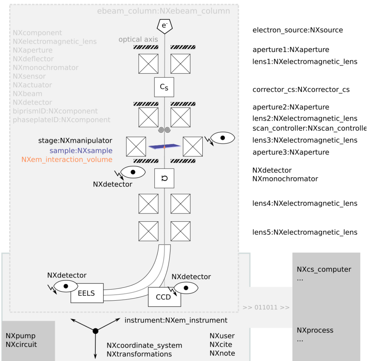
Fig. 3 an example for a (S)TEM The design principles for the SEM as well as the FIB are used for modeling a transmission electron microscope. Noteworthy is that the figure illustrates an optical setup that is a mixture of a conventional TEM and a STEM (again for illustrative purposes). The presence of a scan controller is one characteristic feature of an STEM. Given that a TEM specimen is typically orders of magnitude thinner than a specimen used in an SEM, the electron beam can penetrate the material. This enables investing additional imaging modes and probing other characteristic electron-matter interactions such as electron energy loss spectroscopy. Consequently, additional lenses and components are introduced into the beam path of the exiting electrons.
