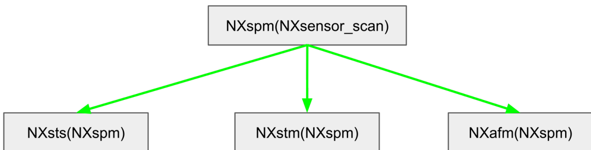
Fig. 11: Inheritance relationship among SPM application definitions.
