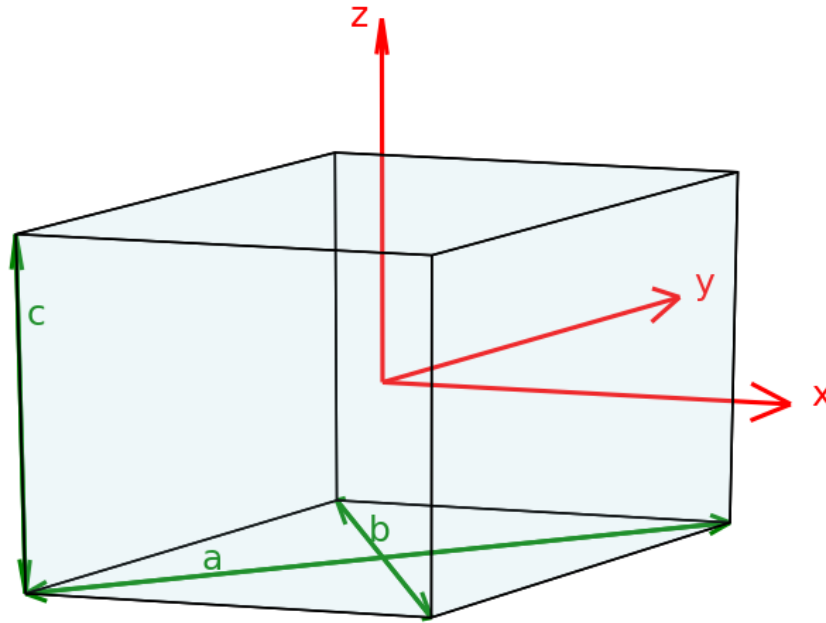
Fig. 15: Gauge volume parameters and coordinate system.
