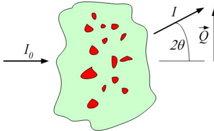
Fig. 13: The \vec{Q} geometry. (full image)
