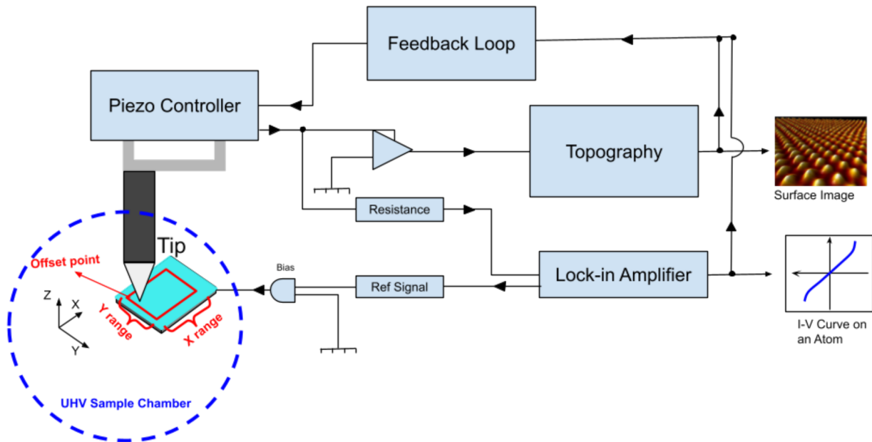
Fig. 10: A schematic diagram of Scanning Tunneling Microscopy (STM) and Spectroscopy (STS) setup generate topography image and I/V curve.
