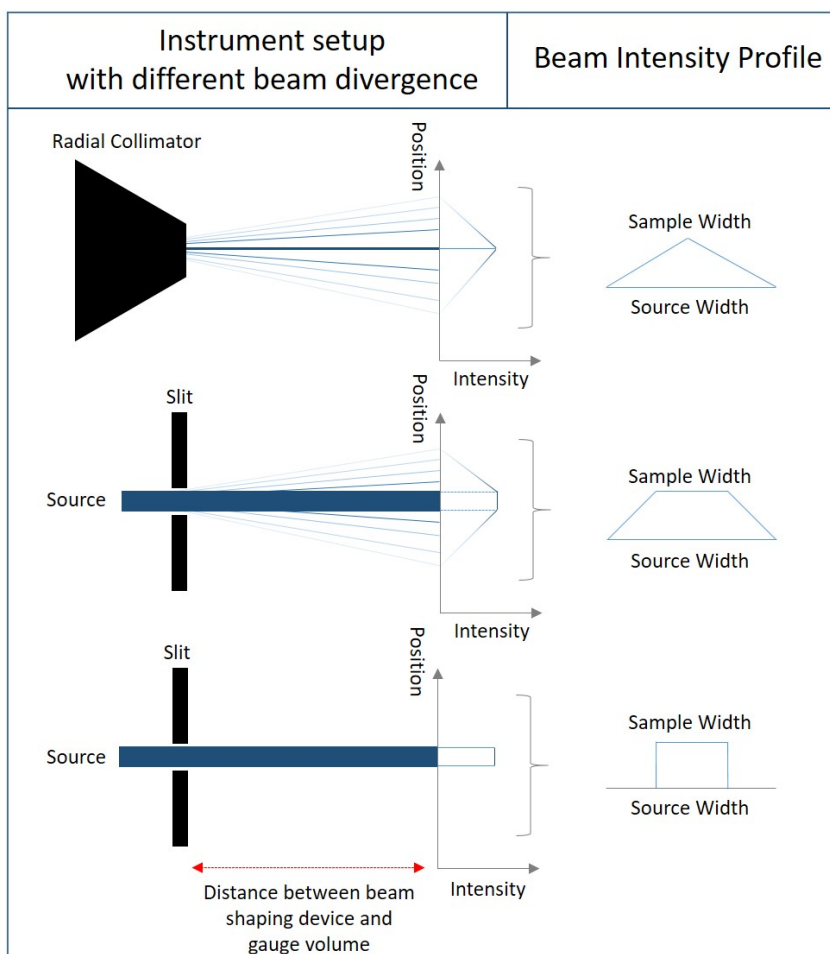
Fig. 14: Some examples for the beam intensity profile. The 1D description of the beam profile on the right can equally be applied for the horizontal and vertical direction for the primary and the secondary side.
