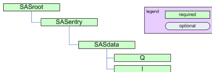
Fig. 12: The minimum requirements for reduced small-angle scattering data. (full image) See below for the minimum required information for a NeXus data file written to the NXcanSAS specification.
