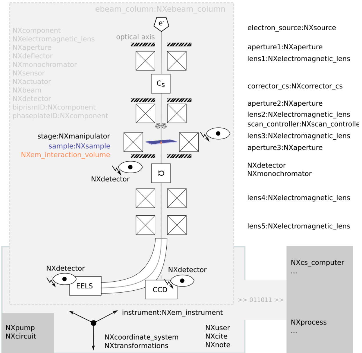
Fig. 3 an example for a (S)TEM The design principles for the SEM as well as the FIB are used for modeling a transmission electron microscope. Noteworthy is that the figure illustrates an optical setup that is a mixture of a conventional TEM and a STEM (again for illustrative purposes). The presence of a scan controller is one characteristic feature of an STEM. Given that a TEM specimen is typically orders of magnitude thinner than a specimen used in an SEM, the electron beam can penetrate the material. This enables investing additional imaging modes and probing other characteristic electron-matter interactions such as electron energy loss spectroscopy. Consequently, additional lenses and components are introduced into the beam path of the exiting electrons.
