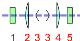
Fig. 17: A complete description of the shapes of the container elements with their orientation relative to the beam and also information on whether they are upstream or downstream of the sample is also therefore important. For example, although the windows 2 and 4 have the same shape, the path taken through them by the beam is very different and this needs to be modelled. Furthermore, it is not inconceivable that windows might move during an experiment and thus the changes to the beampath would need to be accounted for.
