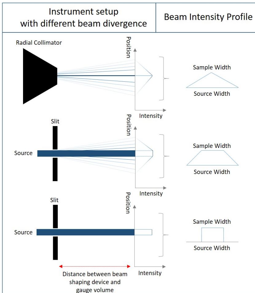
Fig. 12: Some examples for the beam intensity profile. The 1D description of the beam profile on the right can equally be applied for the horizontal and vertical direction for the primary and the secondary side.
