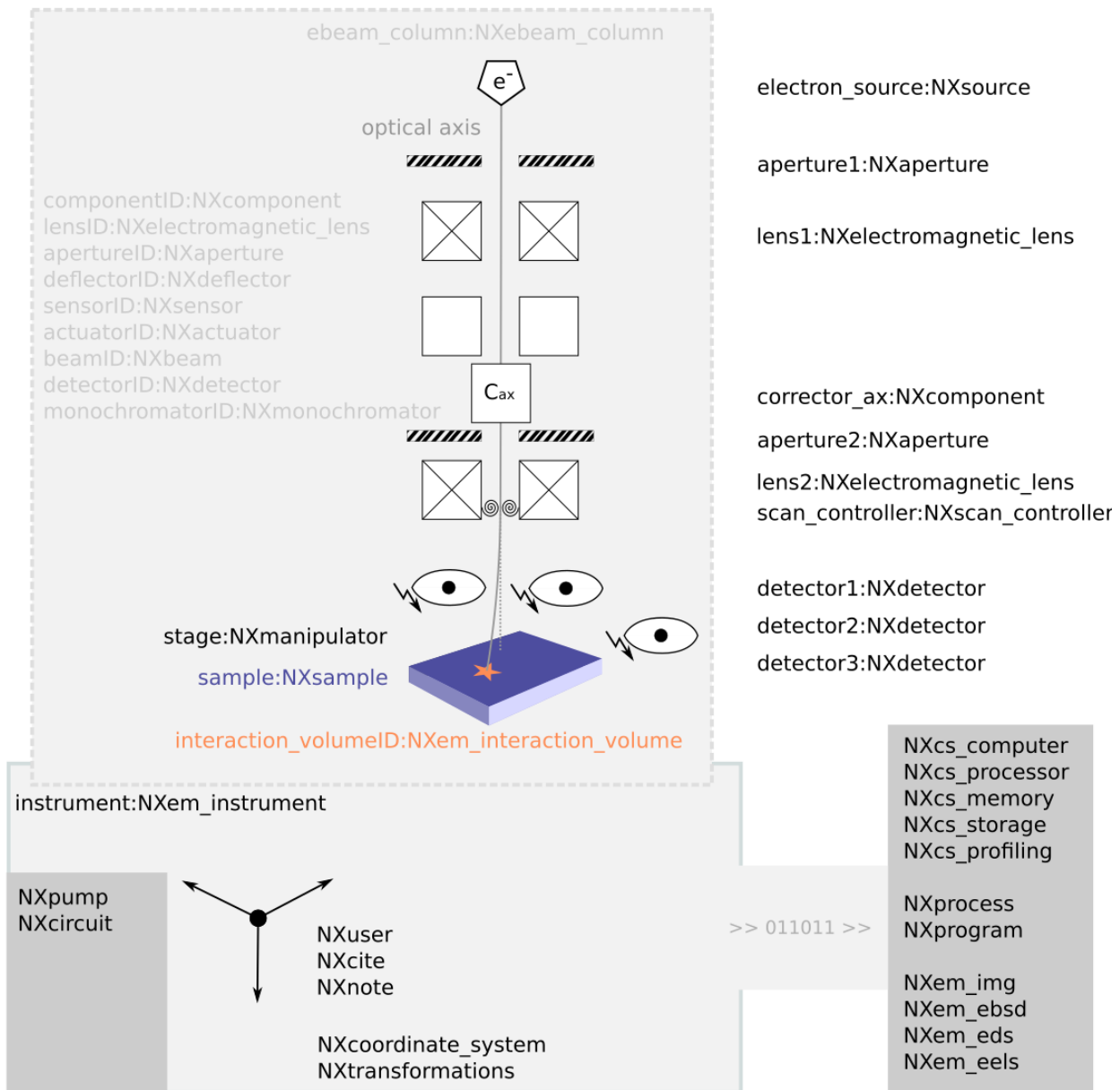
Fig. 1 - an example for an SEM The instrument is constructed from a so-called column, a housing for all technical components such as the electron source, the lenses, like here shown a condenser and an objective lens, respective apertures, and further components, like a stigmator to correct for axial image distortions. The trajectory of the electron beam along the optical axis is simplified for illustrative purposes. In summary, the sample is illuminated by an electron beam that is guided along the optical axis through and past a set of components. A scan controller is used to deflect this beam to illuminate specific locations on the sample surface. In response to the electron-beam sample interaction an interaction volume is formed. Different types of signals are generated that are picked up by different types of detectors. Three detectors are shown as an example. Apart from the column, an SEM has further components: The base classes that are used for modeling these are listed in the lower part of the figure. These document pumps and other hardware, assumptions made such as frames of references and transformations between these frames, and the computing hardware and software tools that are used for controlling the SEM and all its connected components. Using an electron microscope demands processing of data. These processing steps are modeled with instances and specializations of the NXprocess base class. These specializations are used for documenting the parameterization, the results, and the sequence of such processing steps. Examples of method-specific base classes are NXem_ebsd for electron backscat-
