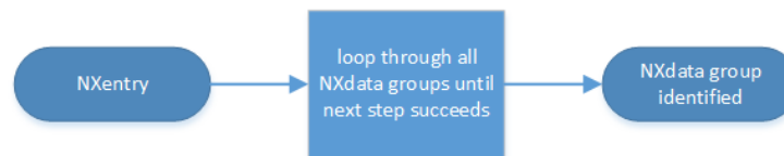
Fig. 10: Find plottable data: pick a NXdata group
