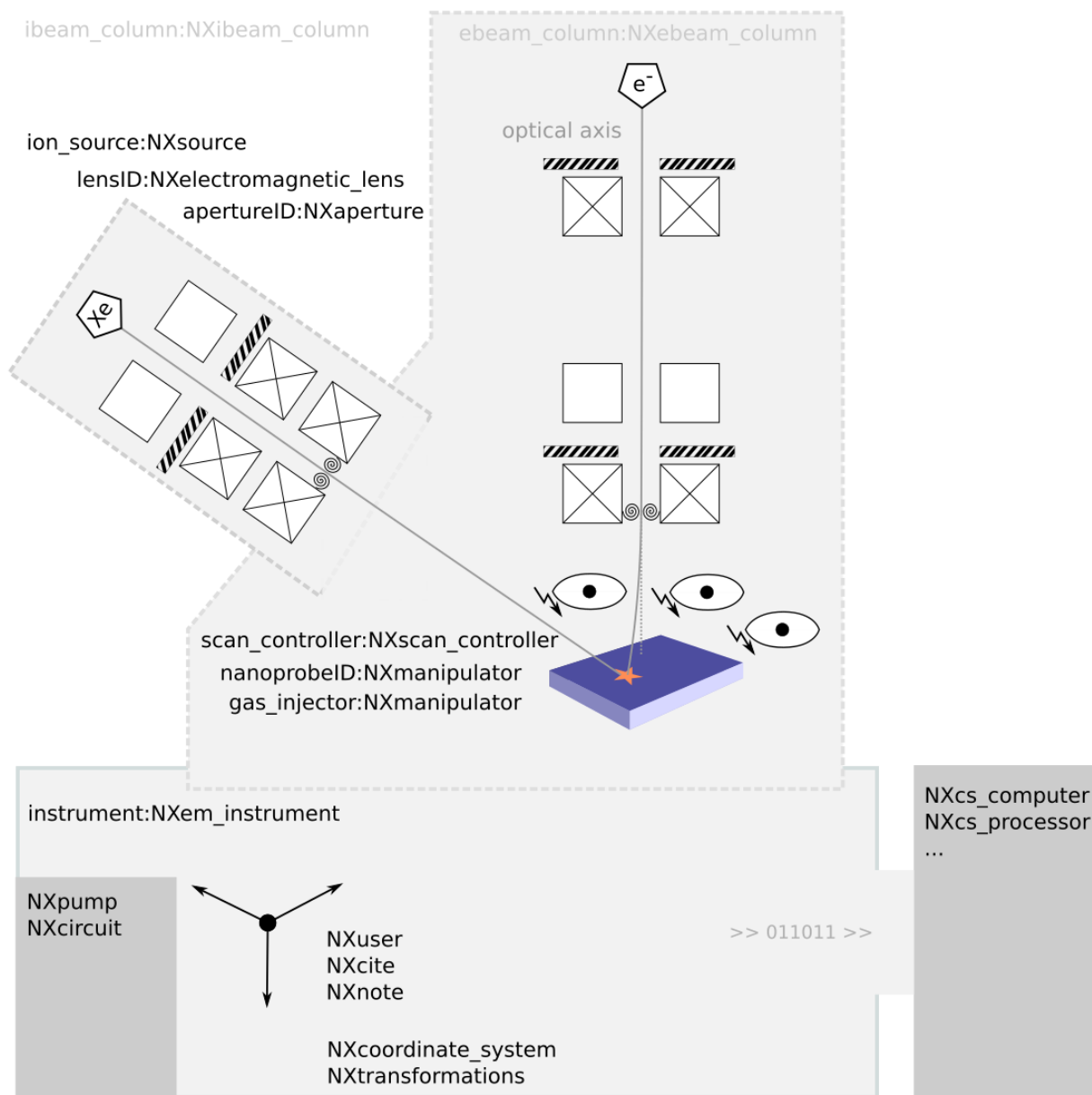
Fig. 2 - an example for an SEM with plasma FIB capabilities Adding or flanging another column to an electron microscope equips it with focused-ion beam capabilities. The design of this NXibeam_column follows the design of the NXebeam_column: A housing with technical components, such as the ion source, lenses, apertures, beam distortion and beam shaping components, and an own scan controller for guiding the ion beam towards the sample surface. Like in Fig. 1, the trajectory of the ion beam is simplified.
