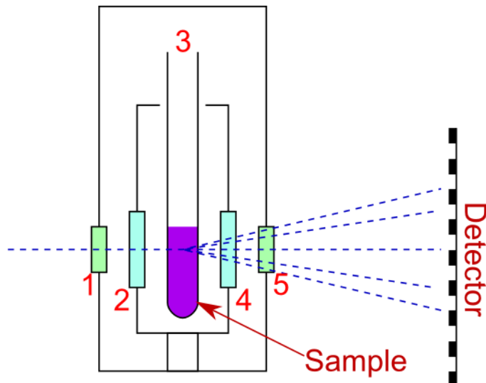
Fig. 16: A hypothetical capillary furnace. The beam passes from left to right (blue dashes), passing through window 1, then window 2, before passing through the downstream wall of the capillary. It is then scattered by the sample with scattered beams passing through the upstream wall of the capillary, then windows 4 and 5. As part of the corrections for a PDF experiment it is necessary to subtract the PDF of the empty container (i.e. each of the windows and the capillary). To calculate the PDF of the empty container it is necessary to have the measured scattering data and to know the nature (e.g. density, elemental composition, etc.) of the portion of the container which the beam passed through.
