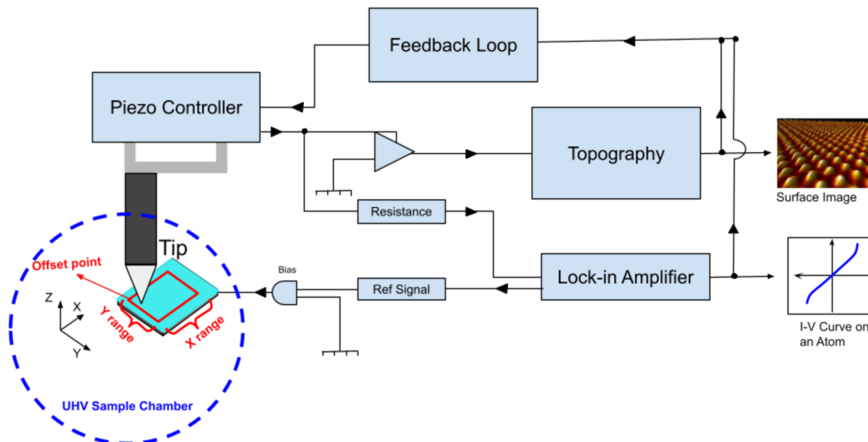
Fig. 14: A schematic diagram of Scanning Tunneling Microscopy (STM) and Spectroscopy (STS) setup generate topography image and I/V curve.
