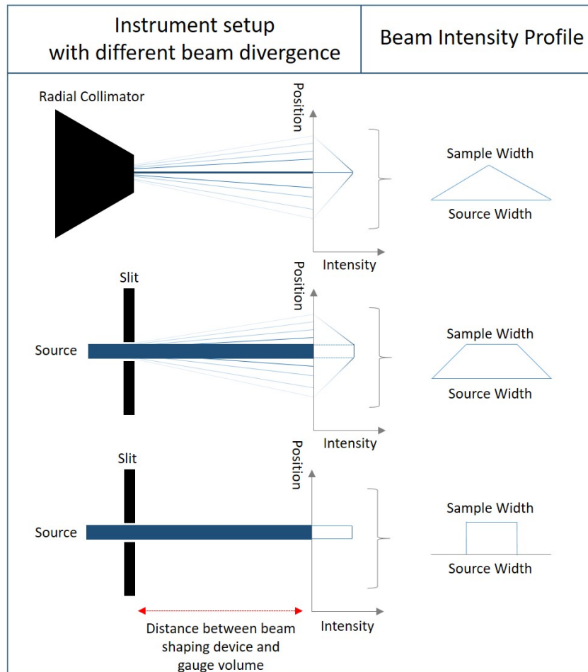
Fig. 13: Some examples for the beam intensity profile. The 1D description of the beam profile on the right can equally be applied for the horizontal and vertical direction for the primary and the secondary side.
