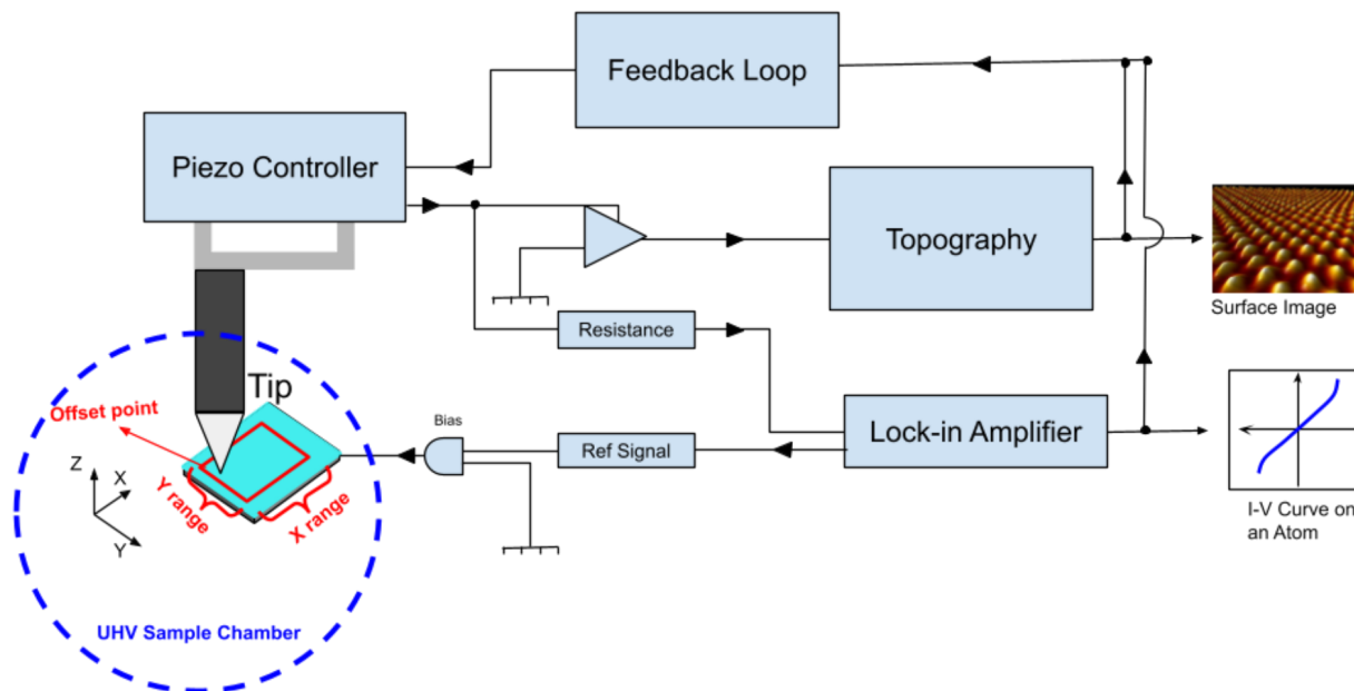
Fig. 15: A schematic diagram of Scanning Tunneling Microscopy (STM) and Spectroscopy (STS) setup generate topography image and I/V curve.
