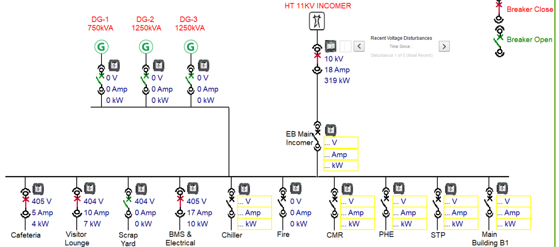
Single Line Diagram Voltage & Current (Click on the meter icon to view the details)
