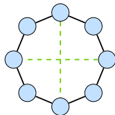
Small-World
