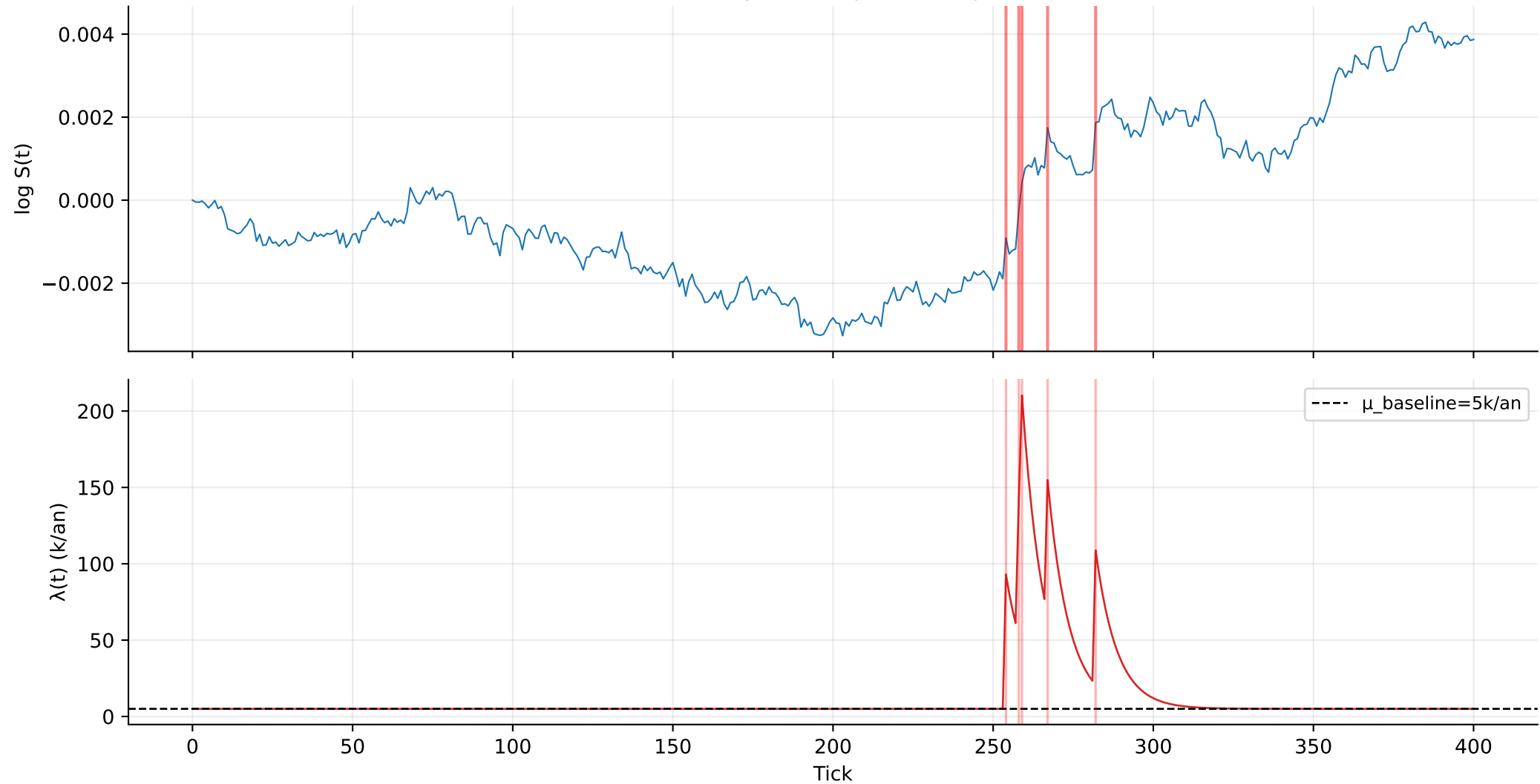
Hawkes auto-excitant | 5 sauts | m=0.50 | clustering visible
