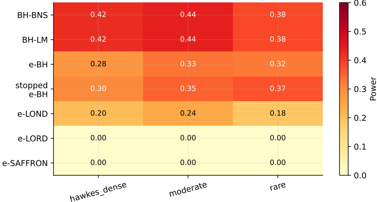
Power ( \pm 2 ticks) | dt=5s, \alpha=0.05 | grid_medium
