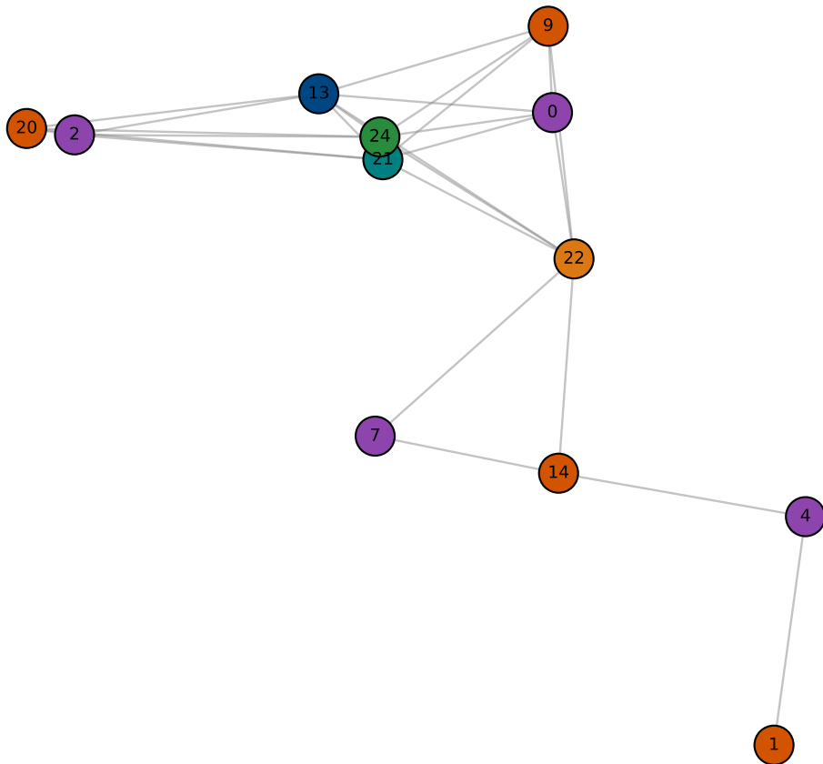
Quantum CG (Dirac-3) \chi = 6
