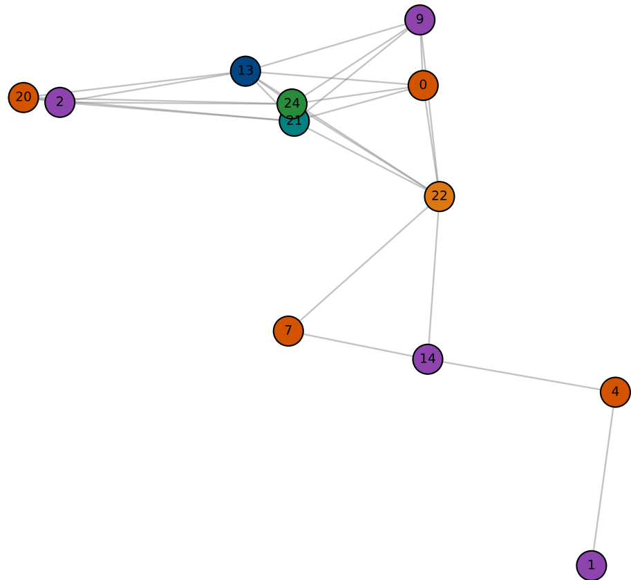
Classical CG \chi = 6
