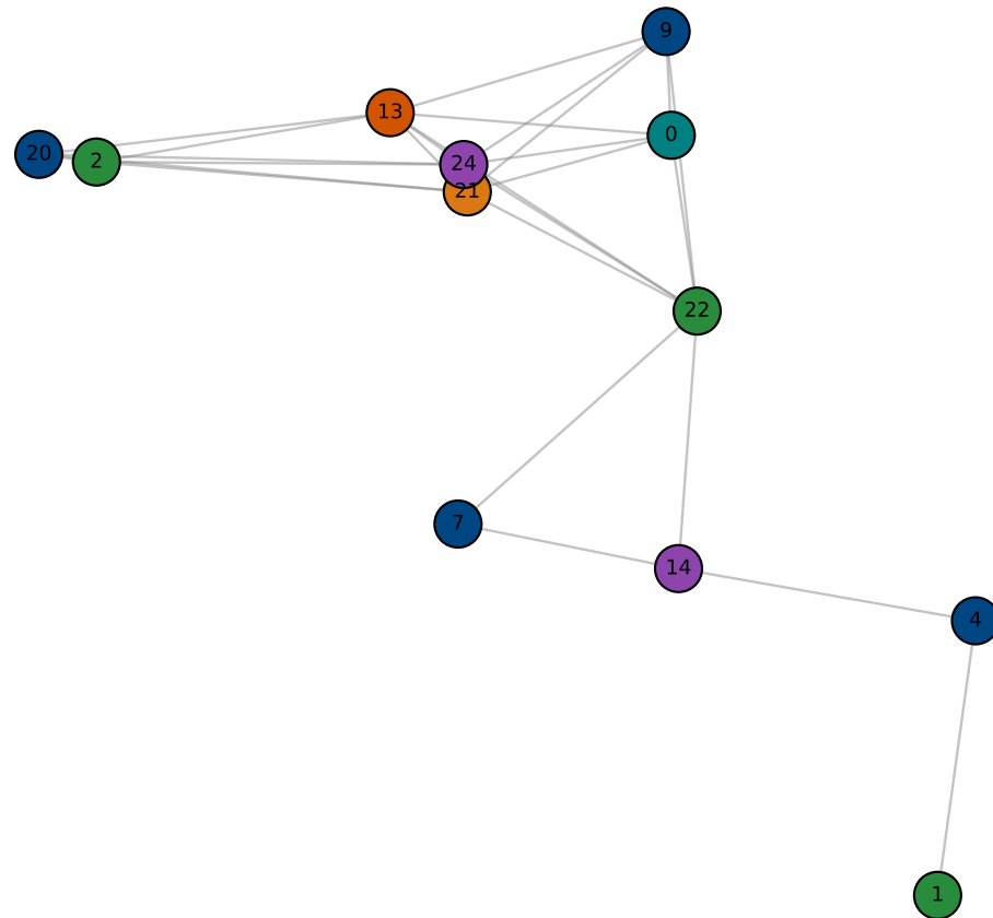
Direct MILP (HiGHS) \chi = 6
