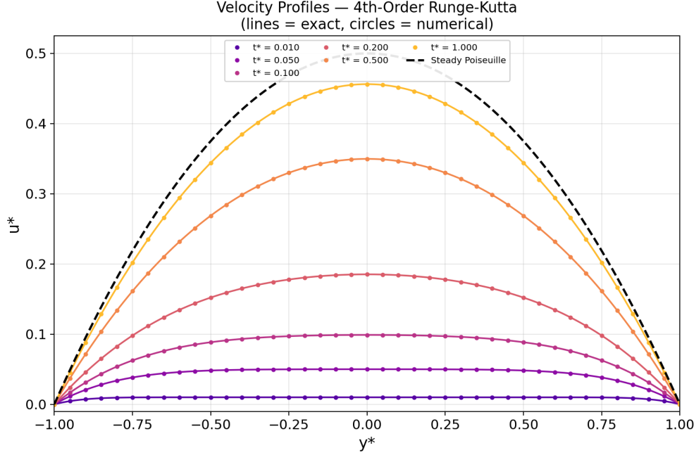
Figure 4: Velocity profiles at six time instants computed using the fourth-order Runge-Kutta method ( N = 40 , r = 0.4 ). Solid lines: exact solution; circles: numerical solution; dashed black: steady state Poiseuille profile.
