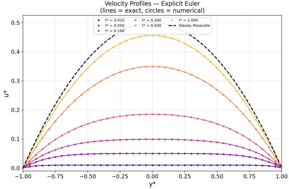
Figure 2: Velocity profiles at six time instants computed using the explicit Euler method ( N = 40 , r = 0.4 ). Solid lines: exact solution; circles: numerical solution; dashed black: steady state Poiseuille profile.
