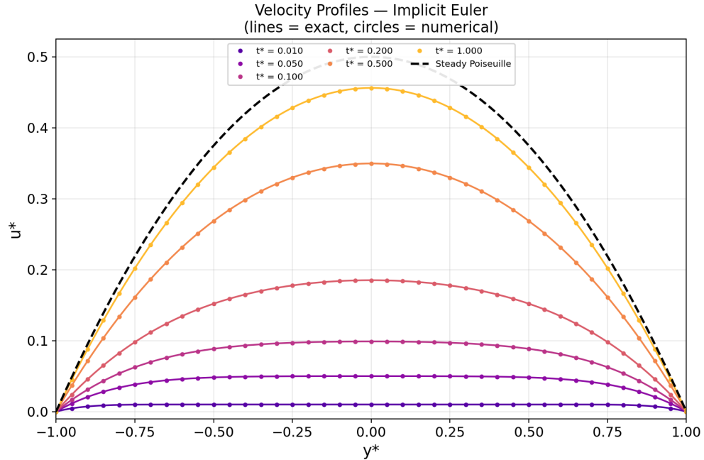
Figure 3: Velocity profiles at six time instants computed using the implicit Euler method ( N = 40 , r = 0.4 ). Solid lines: exact solution; circles: numerical solution; dashed black: steady state Poiseuille profile.
