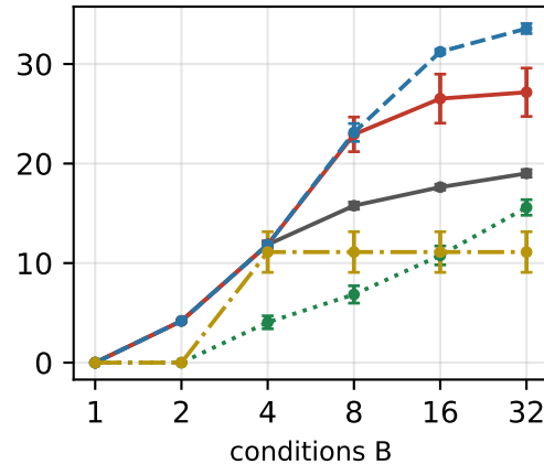
connect_4, win, tau=0.9, certified
