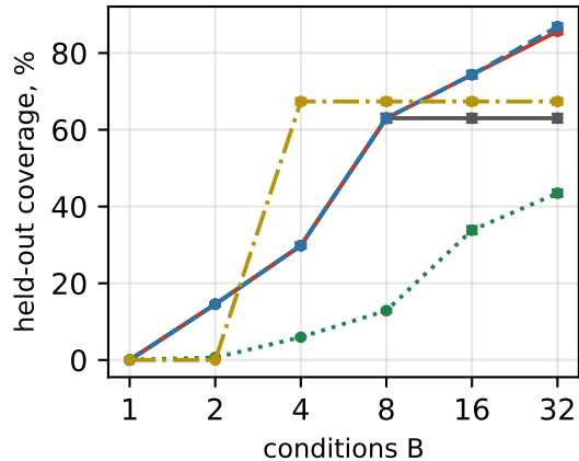
nursery, priority, tau=0.7
