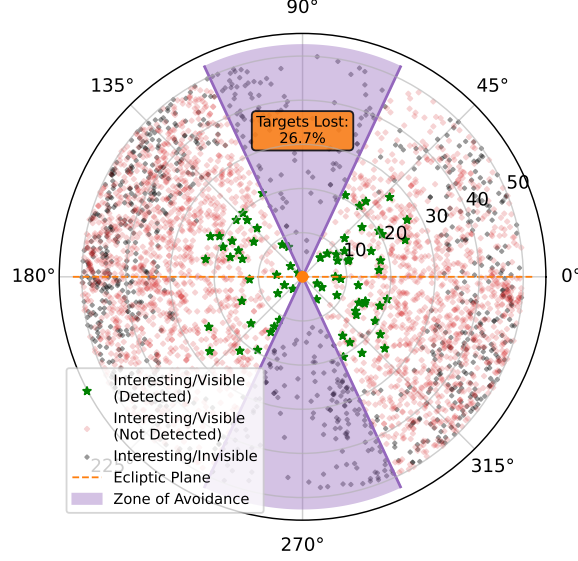
Yields and Cutoffs (65° FoR, Lim. Mag. 7 mag) (Ecliptic Perspective)
