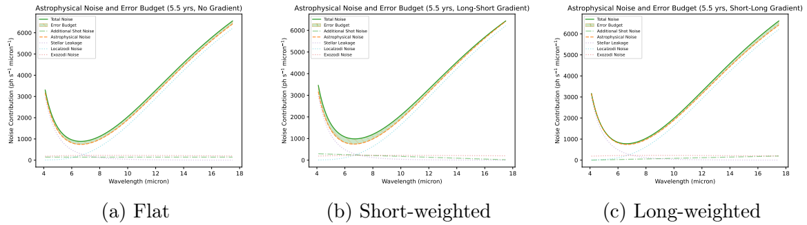
Figure 5.1: Final null-order-two Hab2Max budgets at the common operating point and 5.5-year target. Stellar leakage dominates the short-wave astrophysical background, so the short-weighted ramp admits the largest endpoint.
