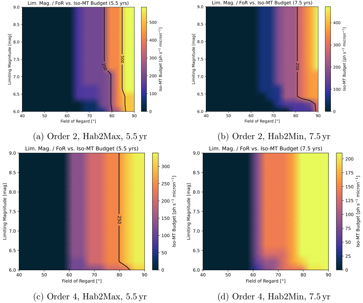
Figure 5.4: Final iso-mission-time flat-budget scans over limiting magnitude and field of regard, with slew time fixed at 12 h. Panels (a) and (b) are the second-order reference array; panels (c) and (d) are the six-aperture fourth-order design of Section 3.4, each sized to its own response peak and at equal total collecting area. Each grid is 15 \times 15 points, so the field-of-regard spacing is 3.6^\circ . Dark regions have no admissible positive budget at the corresponding operating point; the fourth-order design reaches one grid step further into restrictive pointing, at 61^\circ against 65^\circ , in both catalogs. Colour scales differ between panels and peak at 331 and 210 \text{ ph s}^{-1} \mu\text{m}^{-1} for the fourth-order panels against roughly 560 and 460 for the reference, so the fourth-order maps are darker at equal allowance. The recovered grids are tabulated in thesis/reproducibility/stageb_grids.tsv .
