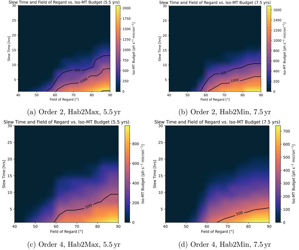
Figure 5.5: Final iso-mission-time flat-budget scans over slew time and field of regard at limiting magnitude 7. Panels (a) and (b) are the second-order reference array, panels (c) and (d) the six-aperture fourth-order design, at equal total collecting area and each at its own baseline prescription. Dark regions have no admissible positive budget: 58.2% and 60.9% of the two fourth-order grids are infeasible at any noise level. Both architectures give the same wedge, feasible only where the slew is short or the field of regard wide; the fourth-order design holds out to 20 h of slew against the reference's 17 h, while peaking lower inside the wedge. Colour scales differ between panels. Recovered grids in thesis/reproducibility/stageb_grids.tsv .
