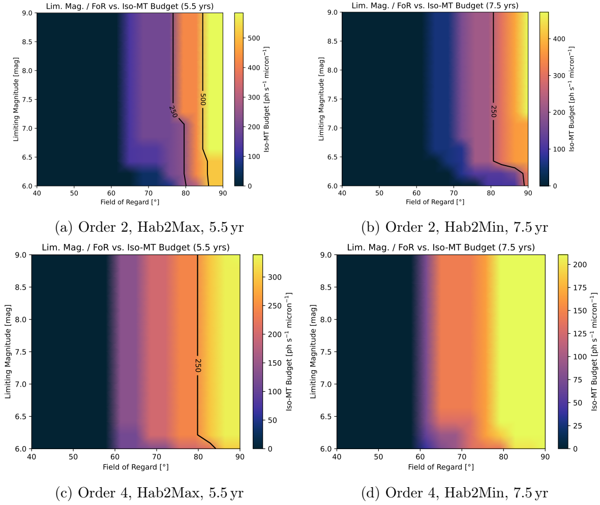
Figure 5.4: Final iso-mission-time flat-budget scans over limiting magnitude and field of regard, with slew time fixed at 12 h. Panels (a) and (b) are the second-order reference array; panels (c) and (d) are the six-aperture fourth-order design of Section 3.4, each sized to its own response peak and at equal total collecting area. Each grid is 15 \times 15 points, so the field-of-regard spacing is 3.6^\circ . Dark regions have no admissible positive budget at the corresponding operating point; the fourth-order design reaches one grid step further into restrictive pointing, at 61^\circ against 65^\circ , in both catalogs. Colour scales differ between panels and peak at 331 and 210 \text{ ph s}^{-1} \mu\text{m}^{-1} for the fourth-order panels against roughly 560 and 460 for the reference, so the fourth-order maps are darker at equal allowance. The recovered grids are tabulated in thesis/reproducibility/stageb_grids.tsv .
