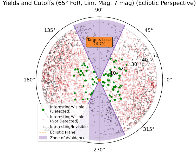
Figure 5.6: Ecliptic view of the final Hab2Max selection at magnitude 7 and FoR 65°. Here “interesting” denotes Experiment-1-eligible targets. The 26.7% value is specific to this catalog and selection.
