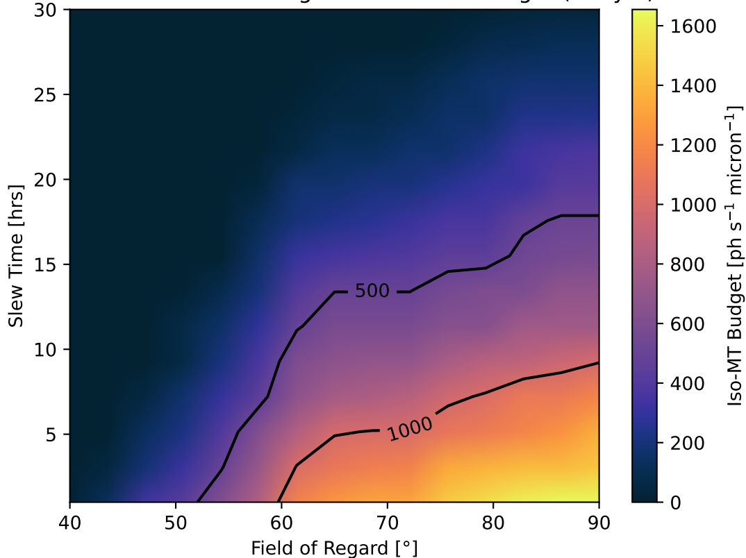
Slew Time and Field of Regard vs. Iso-MT Budget (7.5 yrs)
