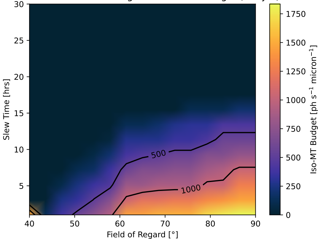
Slew Time and Field of Regard vs. Iso-MT Budget (4.0 yrs)
