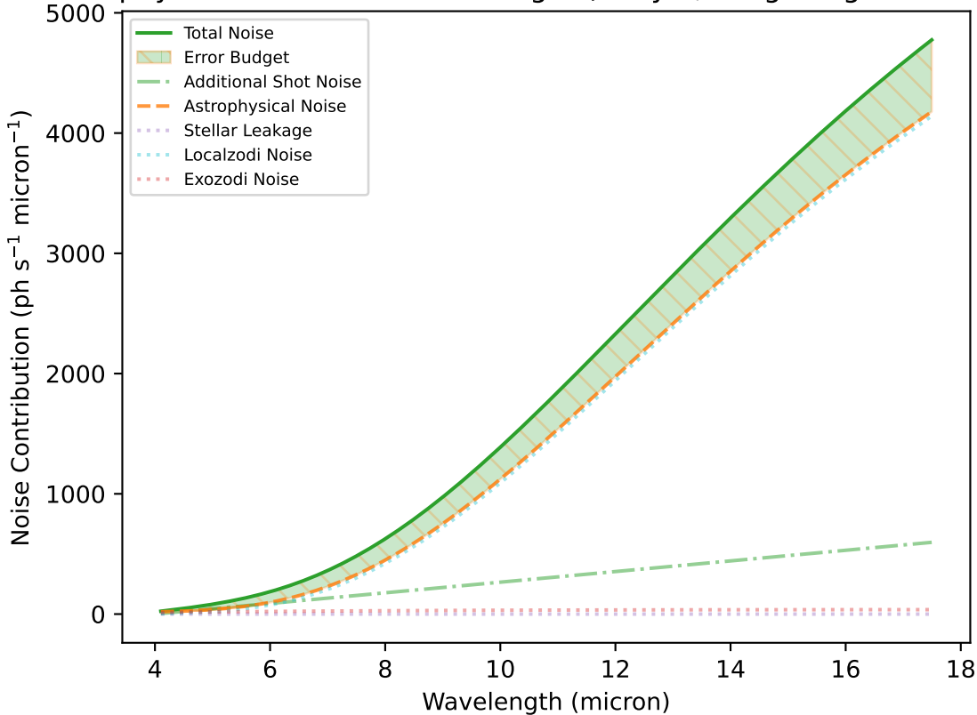
Astrophysical Noise and Error Budget (8.0 yrs, Long-Weighted Budget)
