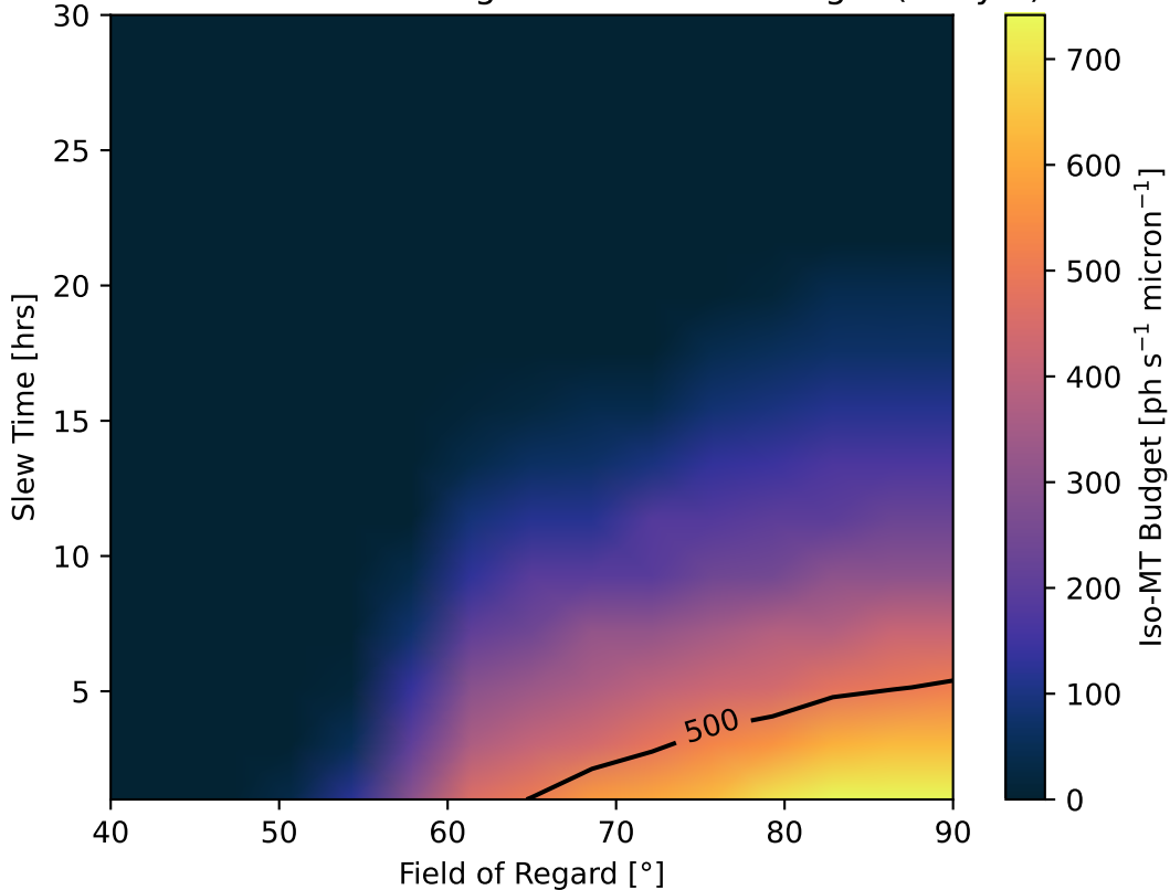
Slew Time and Field of Regard vs. Iso-MT Budget (7.5 yrs)
