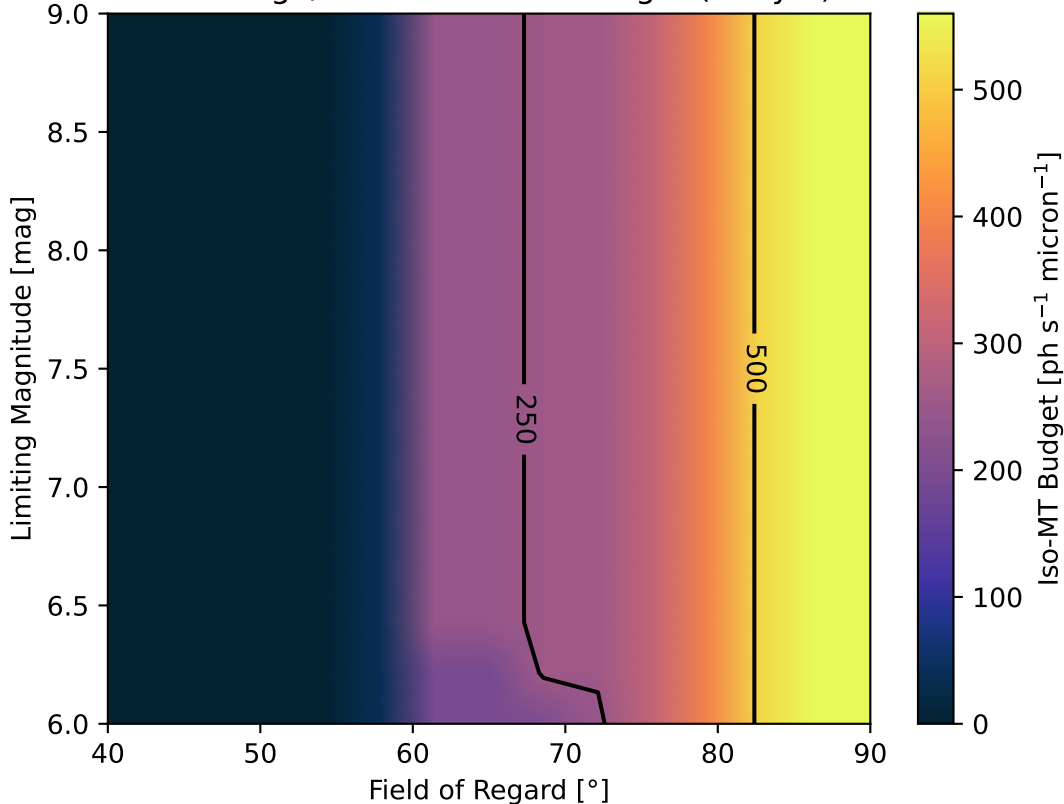
Lim. Mag. / FoR vs. Iso-MT Budget (4.0 yrs)
