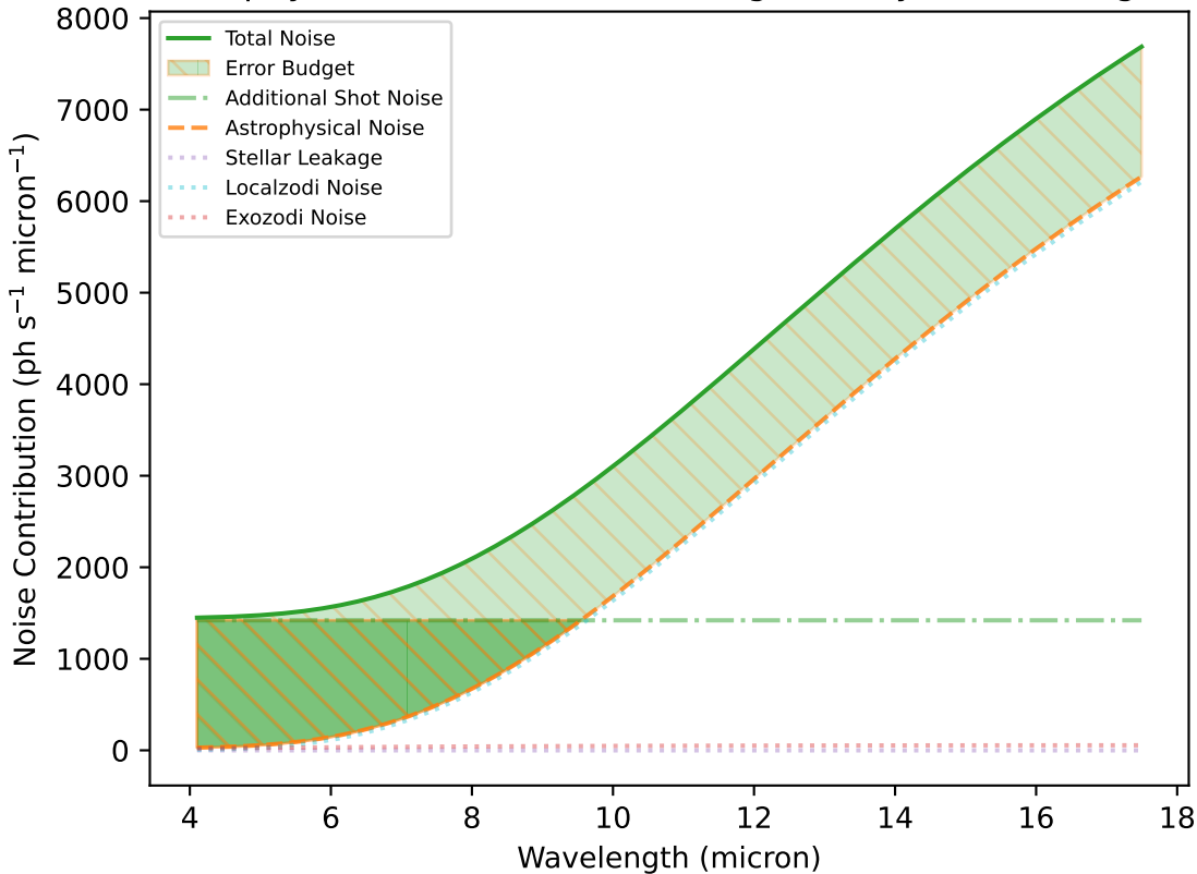
Astrophysical Noise and Error Budget (7.5 yrs, Flat Budget)
