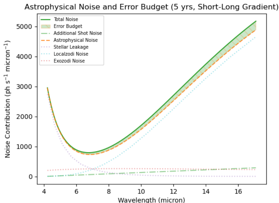
Figure 4.1: Depiction-Construction of the noise-an imposed random-noise budget on top of the astrophysical noisebackground . The dashed green line denotes-is the budget distributionimposed N_I(\lambda) , in this case here a linear distribution-from short to long wavelengths ramp that vanishes at the short-wavelength end of the band and reaches its full amplitude at the long-wavelength end; this is the long-weighted family of Section 5.2. The solid green line stands-for-is the resulting total noise-background including the budget. The-, and the shaded green area between the astrophysical-and total noise-two curves is the actual-error-budgetallowance itself. In this example All three curves are photon-rate spectral densities referred to the budget-pre-efficiency single-output plane, not variances . The amplitude drawn is distributed-such that-the total-one for which the required mission time is exactly five years.
