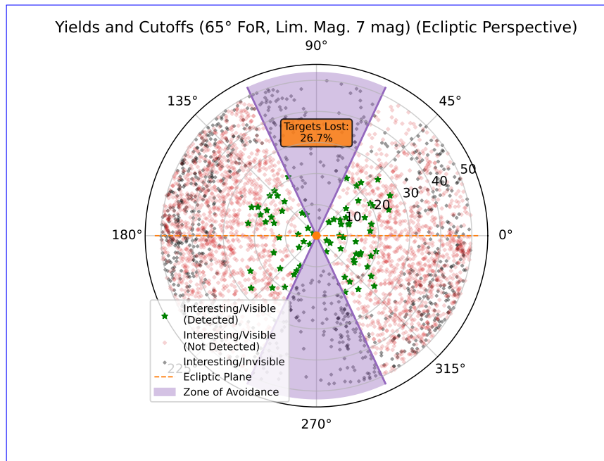
Figure 5.6: Edge-on ecliptic view of the target distribution for final Hab2Max selection at a limiting magnitude of 7 and a field of regard of FoR 65°. The radial coordinate is the distance to the star and the angular coordinate the ecliptic latitude. Green markers are Here “interesting” denotes Experiment-1-eligible targets that are detected, red are interesting but undetected, and black are interesting but rendered invisible by the cuts. The shaded polar wedges are the field-of-regard “zone of avoidance”; at 65° it removes 26.7% of the interesting targets. Detected targets concentrate near the ecliptic plane 26.7% value is specific to this catalog and at small distances selection.
