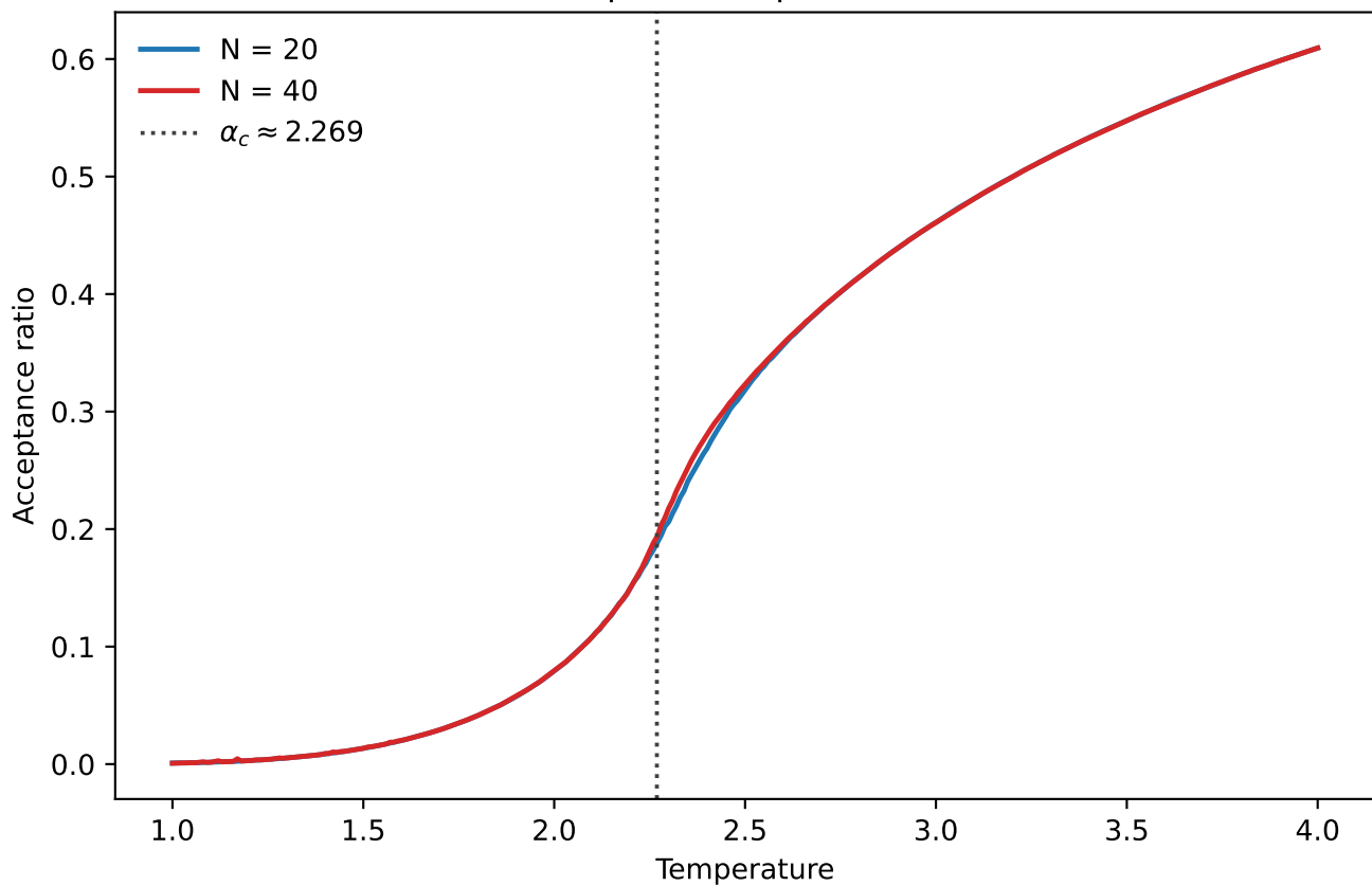
Metropolis acceptance ratio
