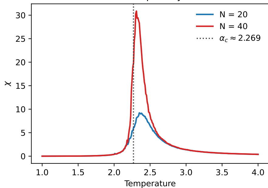
Susceptibility
