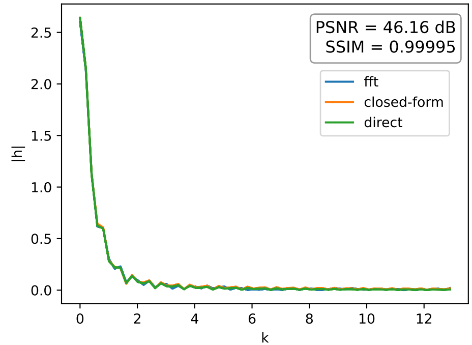
Radial Slice Comparison C_d = 5
