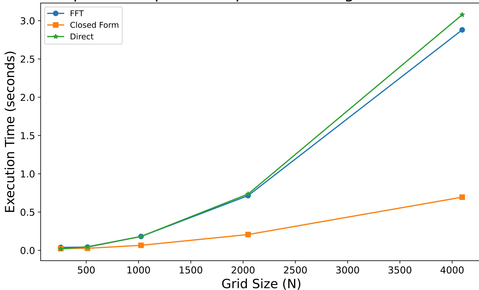
Computation Speed Comparison Averaged Over 20 Runs
