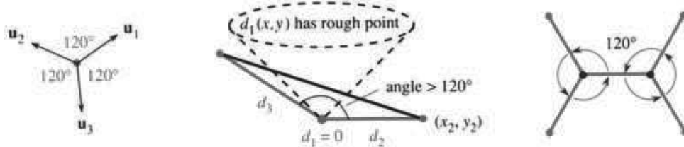
Fig. 13.18 Gradients \mathbf{u}_1 + \mathbf{u}_2 + \mathbf{u}_3 = \mathbf{0} for 120^\circ angles. Corner wins at wide angle. Four corners. In this case two branchpoints are better—still 120^\circ .
