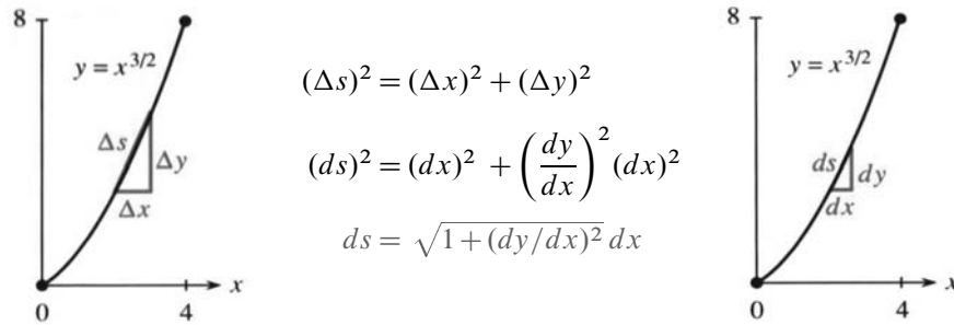
Fig. 8.8 Length \Delta s of short straight segment. Length ds of very short curved segment.
