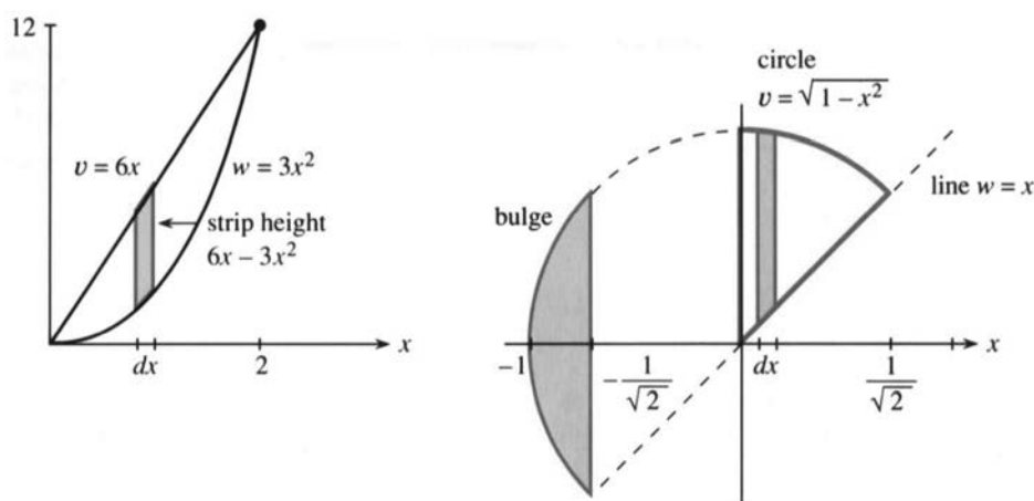
Fig. 8.1 Area between curves = integral of v - w . Area in Example 2 starts with x \geq 0 .
