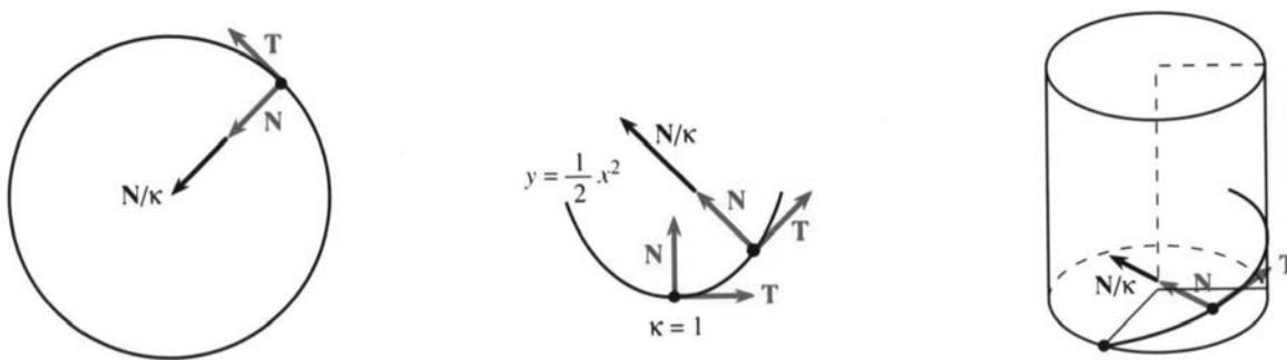
Fig. 12.7 Normal \mathbf{N} divided by curvature \kappa for circle and parabola and unit helix.
