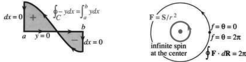
Fig. 15.11 Closed path gives the sign of the area. Nonconservative field because of hole.
