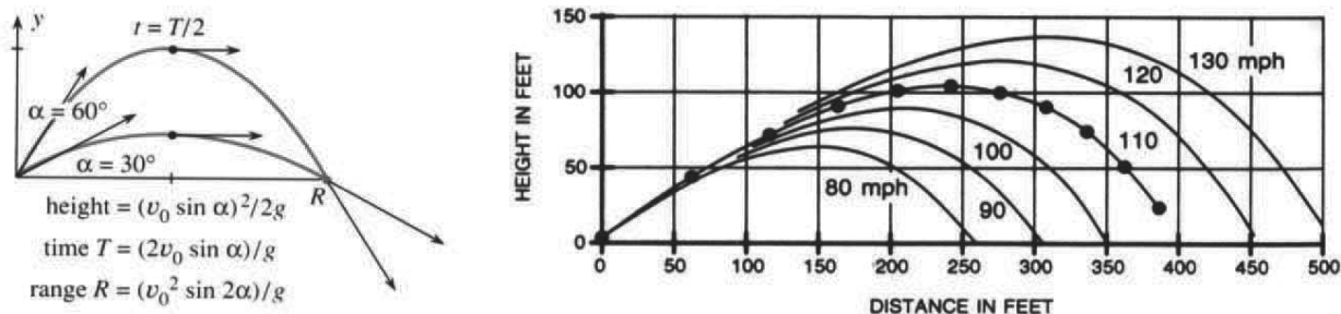
Fig. 12.5 Equal range R , different times T . Baseballs hit at 35^\circ with increasing v_0 . The dots are at half-seconds (from The Physics of Baseball by Robert Adair: Harper and Row 1990).
