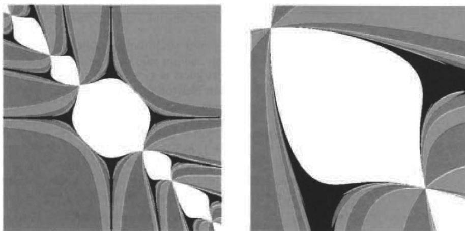
Fig. 13.11 The basins of attraction to (1, 1) , (0, 0) , (-1, -1) , and infinity.
