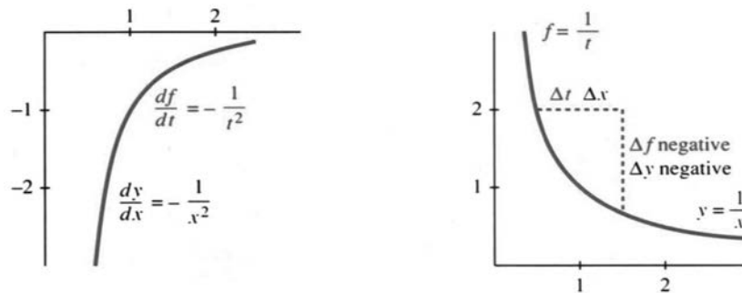
Fig. 2.3 The derivative of 1/t is -1/t^2 . The slope of 1/x is -1/x^2 .
