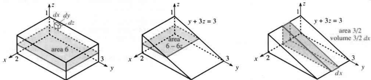
Fig. 14.12 Box with sides 2, 3, 1. The prism is half of the box: volume \int (6 - 6z) dz or \int \frac{3}{2} dx .
