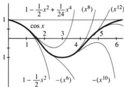
Fig. 10.4 The partial sums 1 - x^2/2 + x^4/24 - \cdots of the cosine series.
