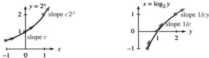
Fig. 6.5 The slope of 2^x is about .7 \cdot 2^x . The slope of \log_2 y is about 1/.7y .
