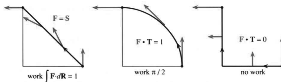
Fig. 15.6 Three paths for \int \mathbf{F} \cdot d\mathbf{R} = \int -y dx + x dy = 1, \pi/2, 0 .
