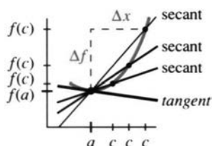
Fig. 2.7 Secants approach tangent as their slopes \Delta f/\Delta x approach df/dx .
