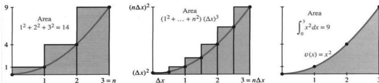
Fig. 5.6 Rectangles enclosing v = x^2 have area \left(\frac{1}{3}n^3 + \frac{1}{2}n^2 + \frac{1}{6}n\right)(\Delta x)^3 \approx \frac{1}{3}(n\Delta x)^3 = \frac{1}{3}x^3 .
