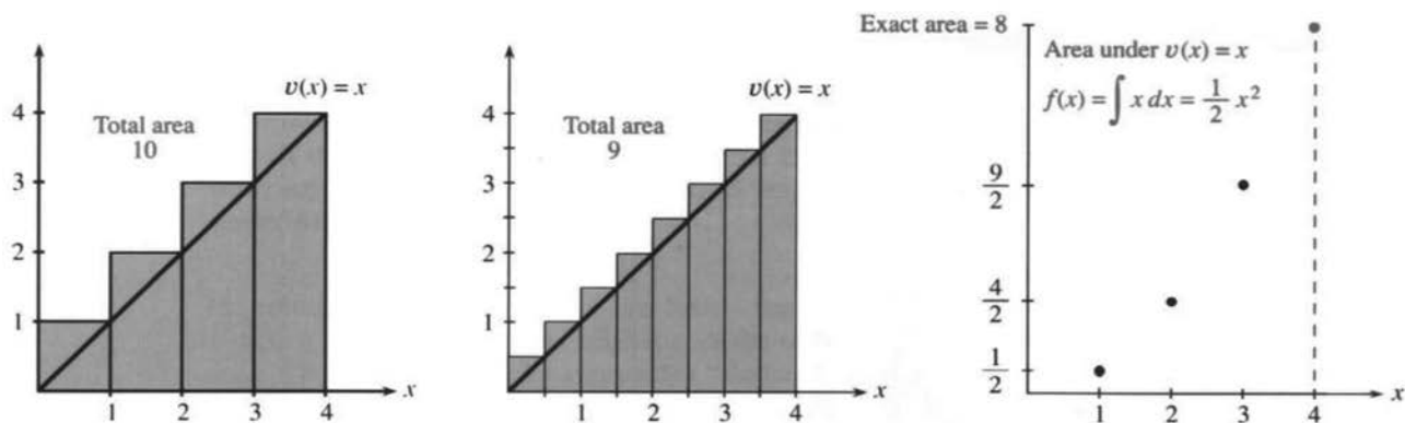
Fig. 5.4 Triangular area 8 as the limit of rectangular areas 10, 9, 8\frac{1}{2} , ....
