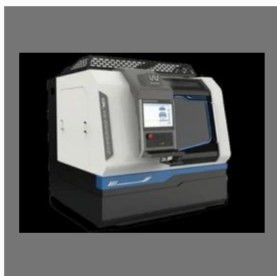
Widma Ecogrind RX5 NEO Tool CNC Grinding Machine
