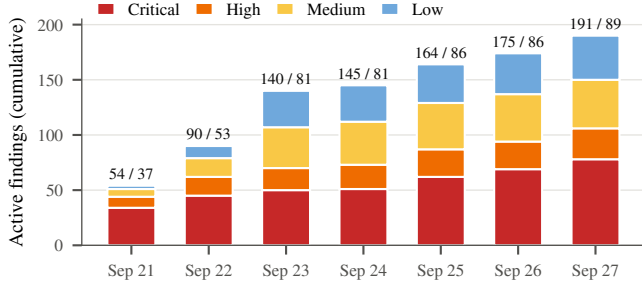
Figure 1. Cumulative active findings by the date shown on each finding, with severities under the final ruleset (bar labels: findings/reports; one Info finding is not drawn). The candidates were published on Sep 20.
