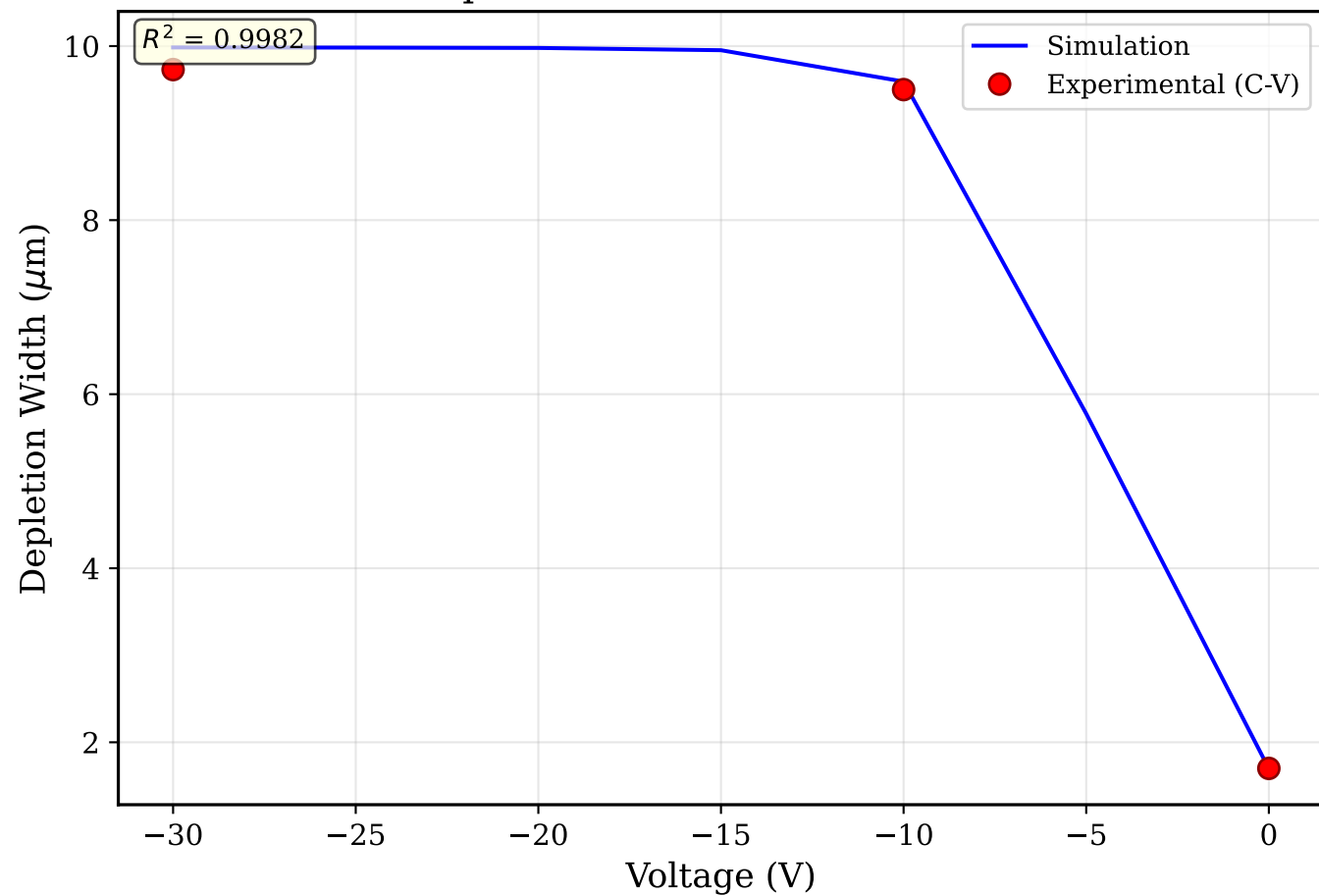
Depletion Width vs Reverse Bias
