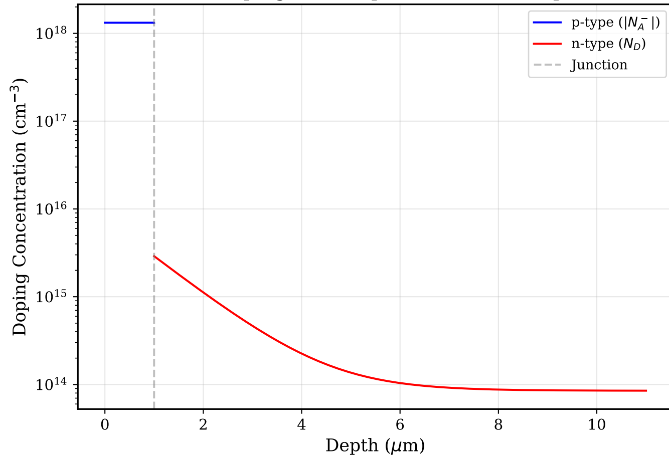
Full Doping Profile (p+ substrate / n- epi)
