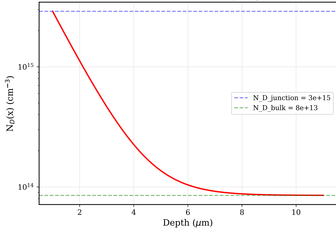
Graded Donor Profile in Epi Layer
