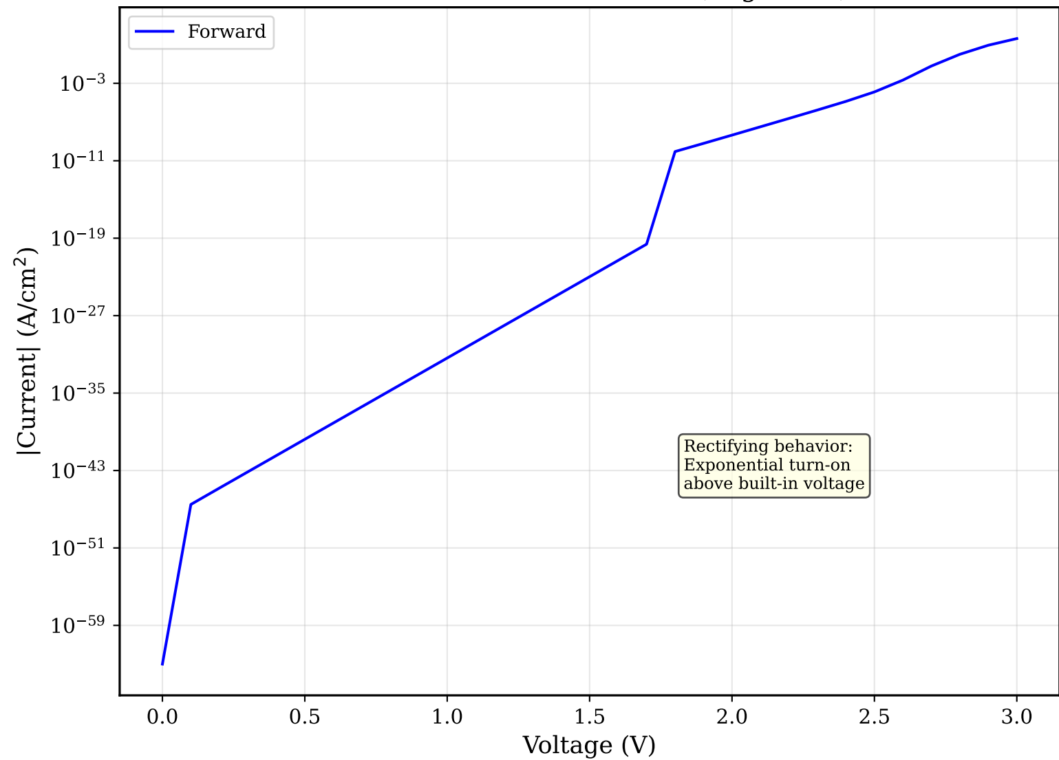
Forward I-V Characteristic (Log Scale)
