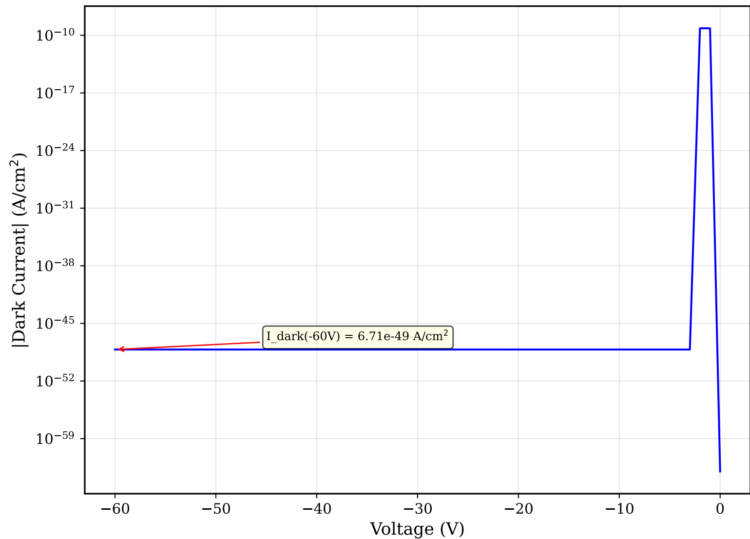
Reverse I-V: Dark Current vs Bias
