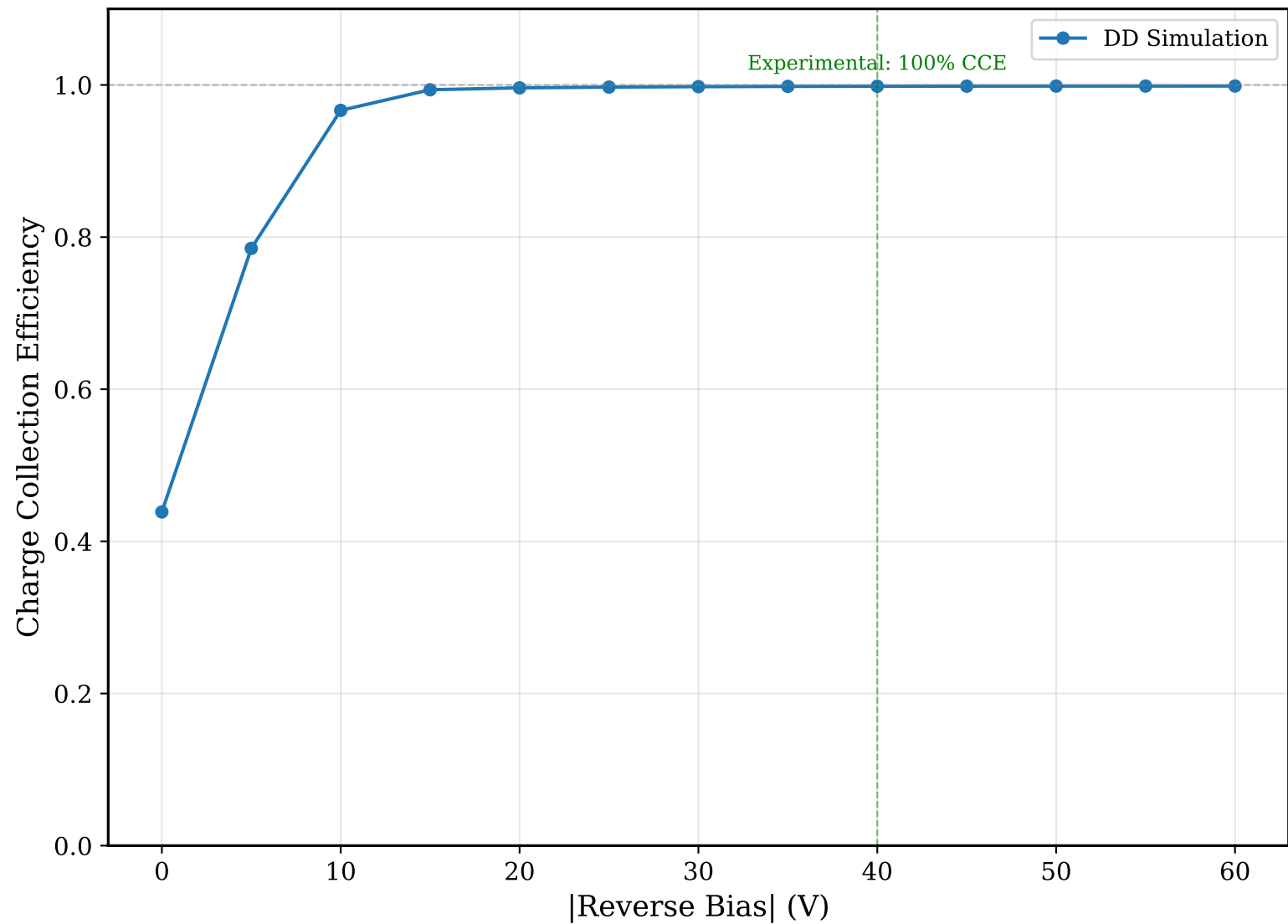
CCE vs Reverse Bias
