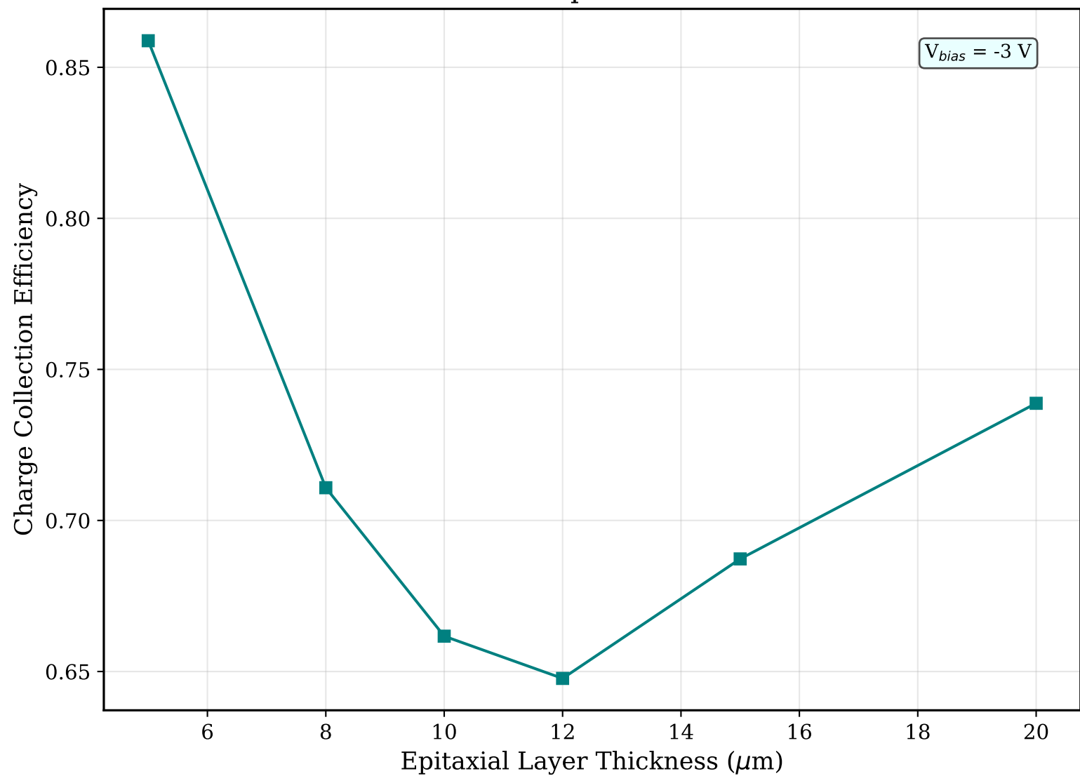
CCE vs Epi Thickness
